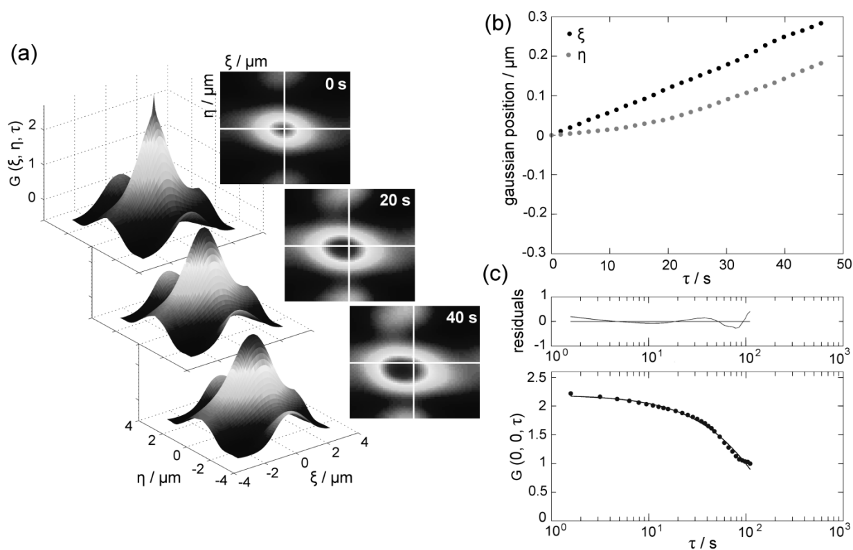
Figure 1. STICS and TICS analyses of PS NP in A549 cells. Image subsections of 64 \times 64 pixels were selected from different regions of the cells shown in Figure 2a. Here region 1 is presented. (a) Spatiotemporal autocorrelation functions G(\xi, \eta, \tau) (STACF) and their contour plot at different time points. (b) Time dependence of the position of the peak of the STACF. (c) The temporal autocorrelation function G(0, 0, \tau) (TACF) was fitted using a diffusion model, considering a fixed flow component as determined by STICS.
