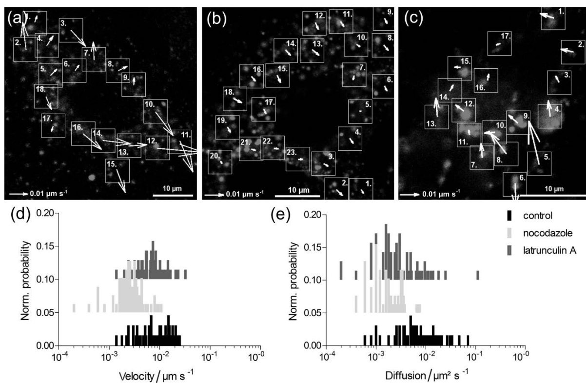
Figure 2. The role of the cytoskeleton in the intracellular dynamics of PS NP transport within A549 cells based on STICS and TICS analyses. Velocity mapping of NP dynamics without treatment (a), and after treatment with 20 \mu\text{M} nocodazole (b) and 500 nM latrunculin A (c). Flow velocities and diffusion coefficients of the presented cells are shown in Table S1. (d-e) Frequency distribution histograms of NP velocity and diffusion coefficient from ROIs of 5 independent cells (expressed as the normalized probability) without (control) and after treatment with cytoskeletal inhibitors.
