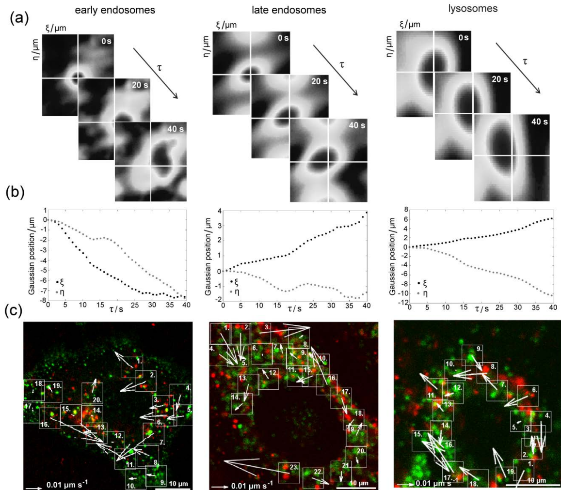
Figure 4. STICCS analyses of correlated motions of PS NP with early endosomes, late endosomes and lysosomes within A549 cells. (a) Contour plot of the cross-correlation peak G(\xi, \eta, \tau) for \tau = 0, 20 or 40 s for early endosomes (ROI 16), late endosomes (ROI 17) and lysosomes (ROI 1). (b) Position of G(\xi, \eta, \tau) as a function of \tau . (c) Dual-channel time series image with PS NP (in red) and cell organelle (in green) together with velocity mapping of NP correlated motions (Figure S2). Effective flow velocities of the cotransport in all ROIs (numbered boxes) are presented Table S2.
