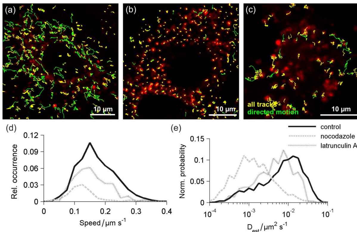
Figure 3. Tracking and quantification of PS NP intracellular dynamics and the role of the cytoskeleton in A549 cells using SPT analysis. (a-c) All PS NP identified tracks (yellow), the identified directed motion sections (green) and PS NP (red) in cells without treatment (a), or treated with 20 μM nocodazole (b) and 500 nM latrunculin A (c) are displayed. The first image of the time series is presented. (d) The distribution of the speed of NP transport over the sections is shown per treatment. The area under the curve represents the relative contribution of directed motion to the overall PS NP dynamics in each condition. (e) From each trajectory an estimator of the diffusion coefficient ( D_{est} ) was determined and the corresponding distribution over all trajectories from each treatment is shown. The normalization is with respect to the total number of trajectories in each condition.
