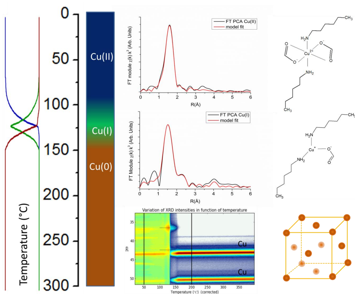
Figure 5: the in-situ reduction of \text{Cu}(\text{hex})_2(\text{HCOO})_2 , consisting out of a stepwise \text{Cu(II)} \rightarrow \text{Cu(I)} \rightarrow \text{Cu(0)} transition according to the displayed concentration profile on the left hand side. The intermediate \text{Cu(I)} and final \text{Cu(0)} structures are determined via EXAFS, XANES and XRD analysis, giving meaning to the observations in coupled TGA-MS and TGA-FTIR analysis.
