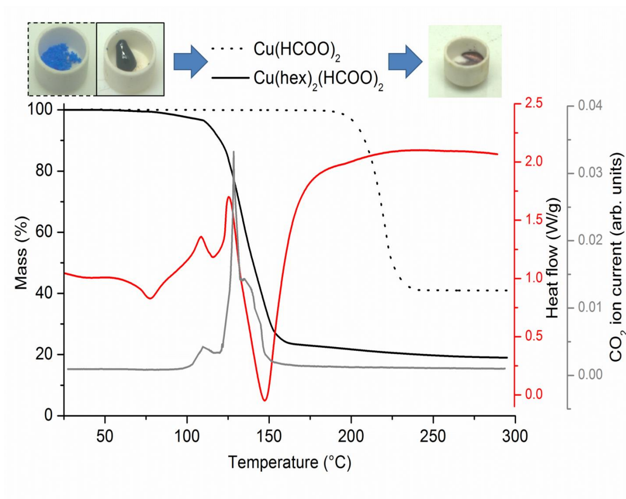
Figure 2: TGA (black curves) of copper formate and its hexylamine complex, together with a simultaneously recorded DSC signal (red, exo-up) and evolved carbon dioxide detection using mass spectroscopy (grey) for the hexylamine adduct. The images on top macroscopically demonstrate the succesful reduction to metallic copper.
