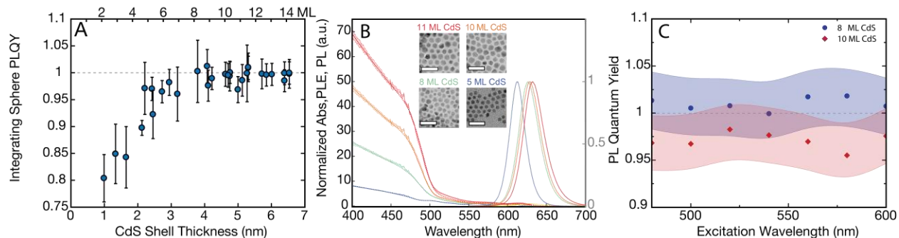
Fig. 1. Characterization of highly emissive CdSe/CdS quantum dots. (A) PLQY for many samples with different shell thicknesses grown with our synthesis procedure. (B) Absorption factor (dotted lines), PLE (shaded regions), and PL spectra (Solid lines) for 5, 8, 10, 11-monolayers CdS shells respectively. Inset: representative transmission electron micrographs, all scale bars are 25 nm. (C) Wavelength-resolved PLQY of 8 and 10-monolayer samples shown in figure 1B. Full characterization (SM4) dataset in figures S1-9.
