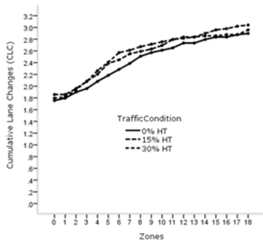
(a) Standard Design
