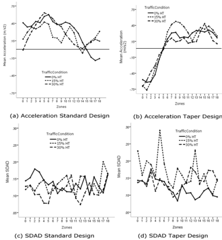
2 Figure 5: Acceleration/deceleration and Standard deviation of acceleration/deceleration profiles for standard and taper design
