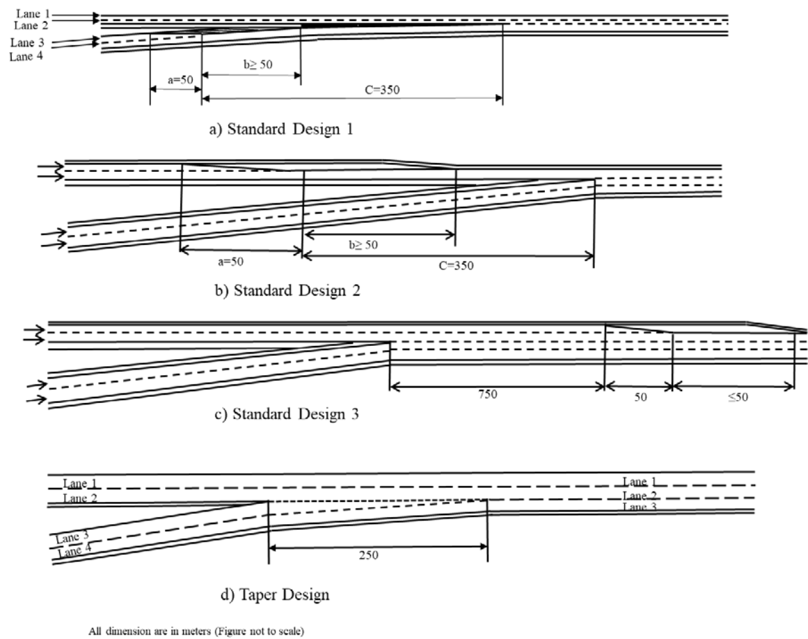
Figure 1: Standard and Taper designs according to Dutch Standards
