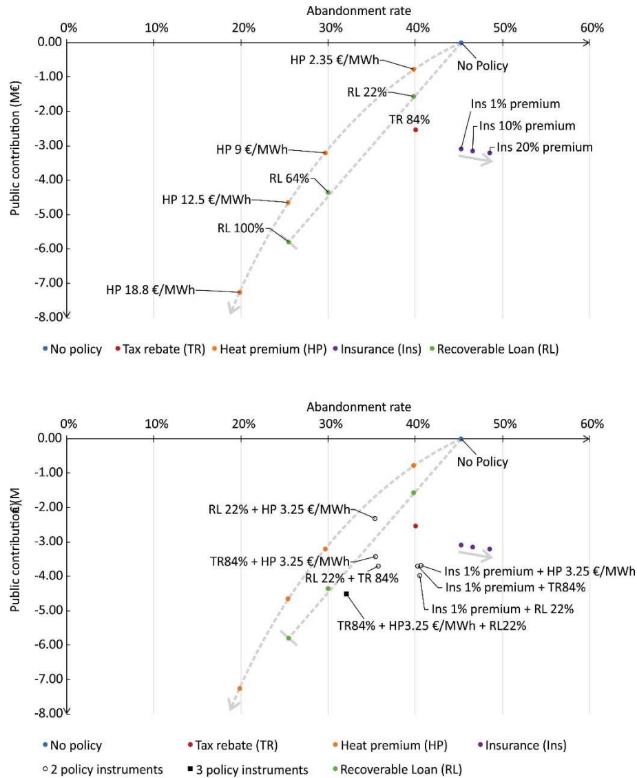
Figure 5. Impact of the different policy instruments on the probability that a geothermal project is abandoned after the first drilling. The upper pane presents the impact and the public contribution of the single policy instruments. In the lower pane, the combinations of policy measures that individually result in an abandonment rate of 40% are added. The public contribution is a cost and therefore results in a negative value.
