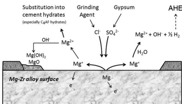
Figure 12: Model of magnesium alloy anodic corrosion behavior in Portland cement paste (left) and geopolymer paste (right)- AHE indicates the Anodic Hydrogen Evolution 122 .
