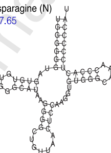
Serine (S1) -25.94
