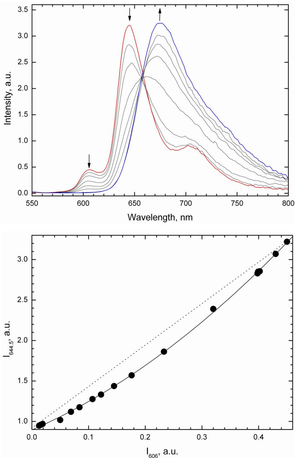
Fig. 2. (top) Fluorescence spectra of the H_3AB_2 meso-pyrimidinylcorrole measured over the course of the titration with H_2SO_4 in ethanol ( \lambda_{exc} = 465 nm). Arrows indicate the direction of intensity changes during the titration. (bottom) Intensity vs. intensity plot demonstrating the changes in the proportion between the excited singlet S_1 state concentrations of the two NH tautomers over the course of the titration. The dotted straight line indicates the hypothetic proportion when the two corrole NH tautomers are protonated at the same rate. See text for details.
