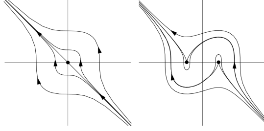
FIGURE 7. From a fake saddle to two cusps
