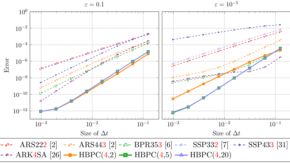
Figure 2: Comparison among different IMEX one-derivative Runge-Kutta schemes and the scheme \text{HBPC}(4, k_{\max}) with k_{\max} = 2 , k_{\max} = 5 , and k_{\max} = 20 . Numerical results for van der Pol equation (3) and (18) with \varepsilon = 0.1 (left) and \varepsilon = 10^{-5} (right). Plotted is the error e_{\Delta t} versus \Delta t . The order of the IMEX Runge-Kutta schemes can be seen from the red digit in the legend.
