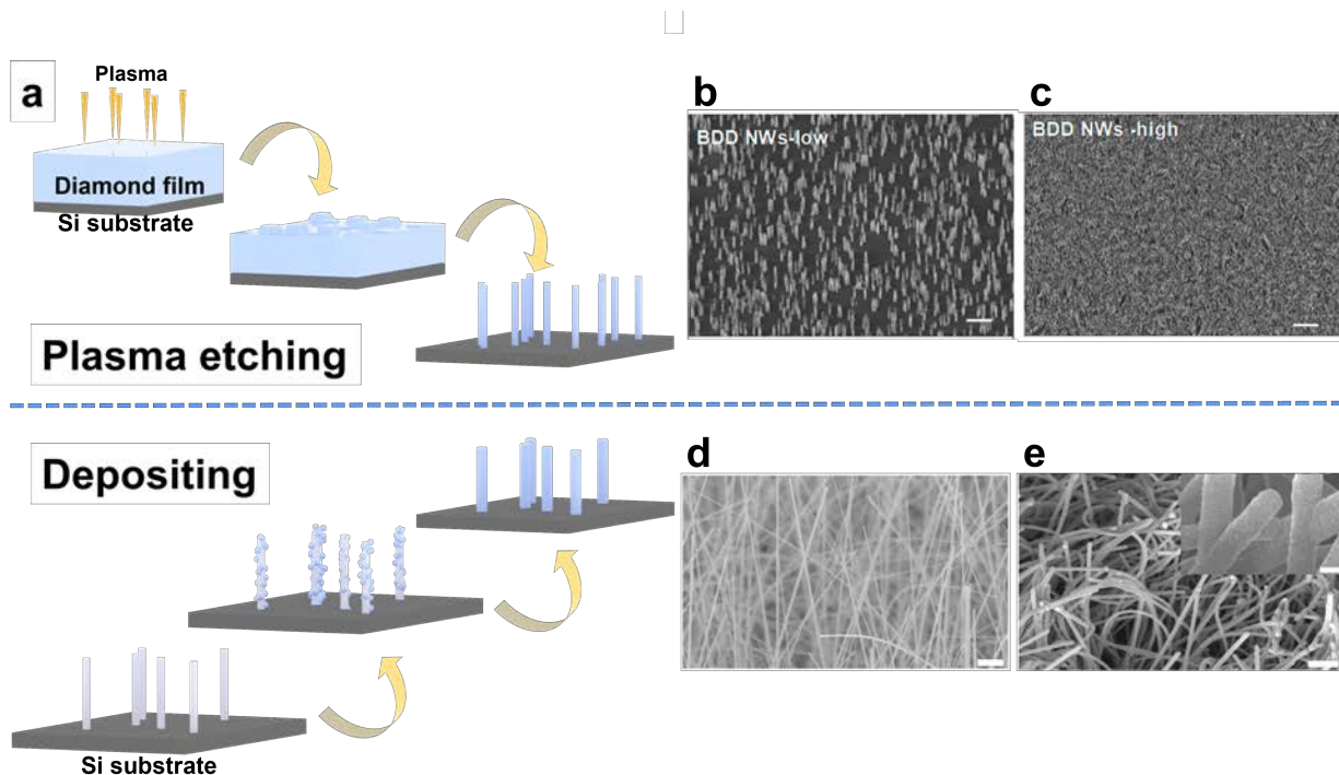
Figure 1. (a) schematic of two kinds of tactics to synthesize DNWs; (b-c) SEM images of BDD NWs in low (b) and high (c) density [23] ; Reproduced under terms of the CC-BY license. [23] Copyright 2017, the Authors, published by American Chemical Society. (d-e) SEM images of Si (d) nanowires and DNWs (e) depositing on Si substrate [2b] ; Reproduced with permission. [2b] Copyright 2017, Elsevier Ltd.
