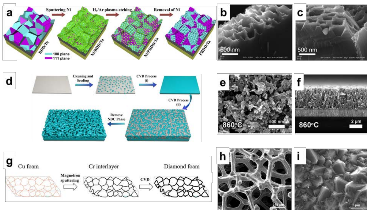
Figure 11. (a-c) (a) schematic of the synthesis of porous diamond structure through etching with, Ni particles acted as catalyzer; SEM images of (111) planes (b) and (100) planes (c) after etching [12c] ; Reproduced with permission. [12c] Copyright 2018, Elsevier Ltd. (d-f) (d) schematic of the synthesis of porous diamond structure on SiC substrate; SEM images of porous BDD films from top view (e) and front view (f) [144] ; Reproduced with permission. [144] Copyright 2022, Elsevier Ltd. (g-i) (g) schematic of the synthesis of porous diamond structure on Cu foam substrate; SEM images of diamond foam from lower magnifications (h) to high magnifications (i) [145] ; Reproduced with permission. [145] Copyright 2019, Elsevier Ltd.
