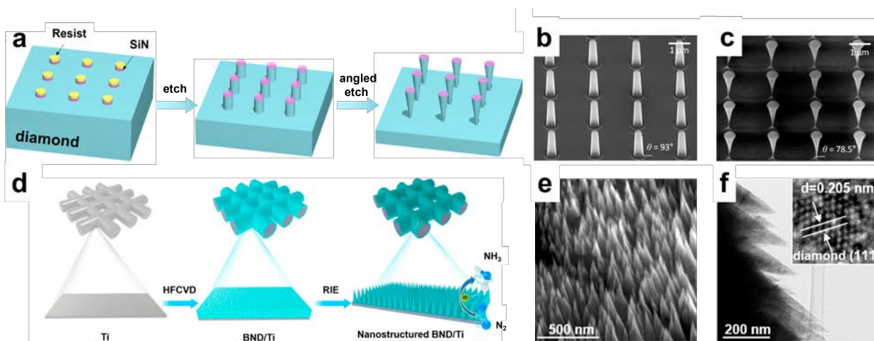
Figure 4. (a-c) (a) schematic of the synthesis of diamond nanorods and diamond inverted nanocones; SEM image of diamond nanorods (b) and diamond inverted nanocones (c) [58]; Reproduced under terms of the CC-BY license.[58] Copyright 2020, the Authors, published by American Chemical Society. (d-f) (d) schematic of the synthesis of diamond nanocones on Ti meshes; high-magnification SEM image (e) and TEM image (f) of it, the inset was HRTEM image [59]; Reproduced under terms of the CC-BY license.[59] Copyright 2020, the Authors, published by American Chemical Society.
