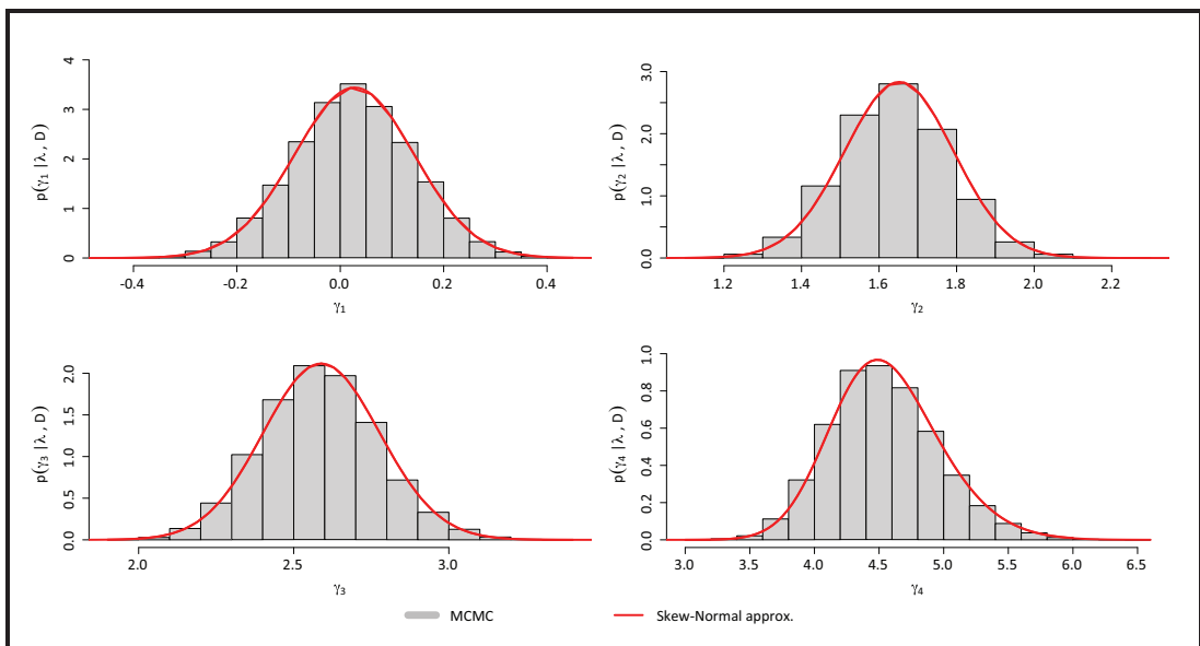
Figure 5 ESS dataset: approximated marginal posterior density for (\gamma|\lambda, \mathcal{D}) compared to MCMC samples when \lambda = \hat{\lambda} .
