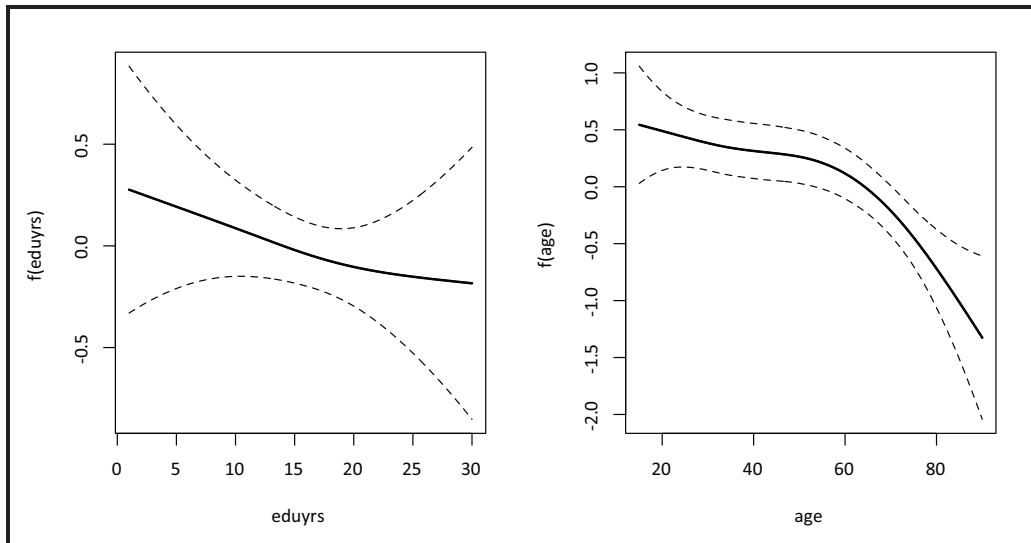
Figure 2 ESS dataset: fitted additive terms for eduysrs and age with pointwise 95% credible intervals: this suggests a growing hostility to homosexuality beyond the age of 60, while it appears that the number of completed years of education does not play a statistically significant role.
