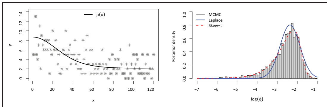
Figure 1 Left panel: Count data ( n = 120 ) generated using a negative binomial \text{NB}(\mu(x), \phi) with \phi^{-1} = 6 . Right panel: Histogram of a MCMC sample for \log \phi compared to Laplace (solid) and skew- t (dashed) approximations.
