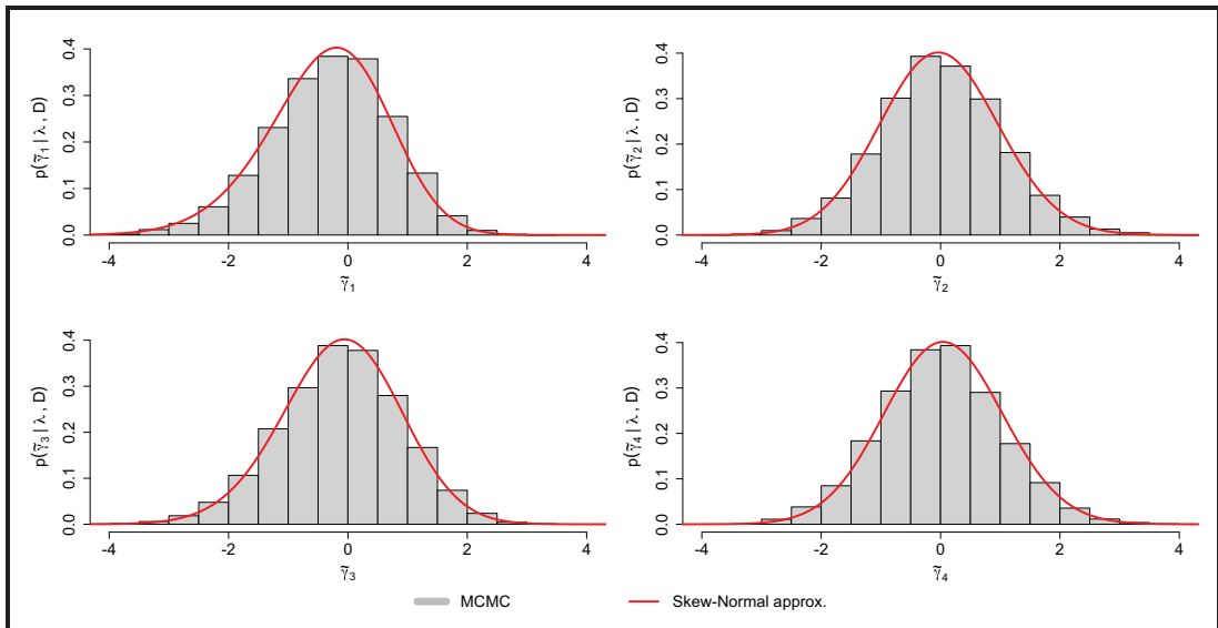
Figure 4 ESS dataset: approximated marginal posterior density for (\tilde{\gamma}|\lambda, \mathcal{D}) compared to MCMC samples when \lambda = \hat{\lambda} .
