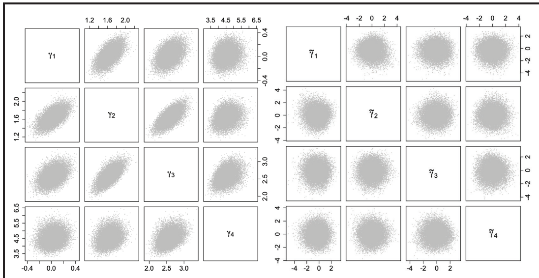
Figure 3 ESS dataset: scatterplots of the MCMC samples for (\boldsymbol{\gamma}|\boldsymbol{\lambda}, \mathcal{D}) and (\tilde{\boldsymbol{\gamma}}|\boldsymbol{\lambda}, \mathcal{D}) when \boldsymbol{\lambda} = \hat{\boldsymbol{\lambda}} .
