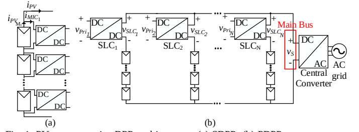
Fig. 1. PV systems using DPP architectures: (a) SDPP, (b) PDPP.
