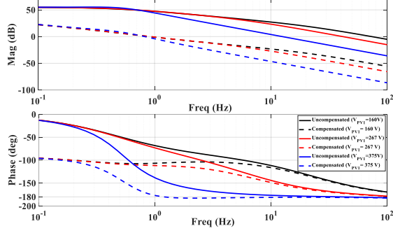
Fig. 16. Bode plot of the compensated and uncompensated open-loop D_5(s) to V_{VB}(s) transfer function at different operating points.
