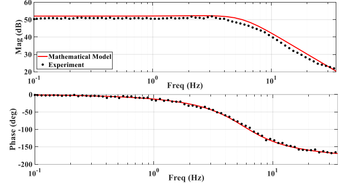
Fig. 13. D_S(s) to V_{VB}(s) transfer function. The input used for system identification is a two-period 11-bit PRBS with clock frequency of 100 Hz.
