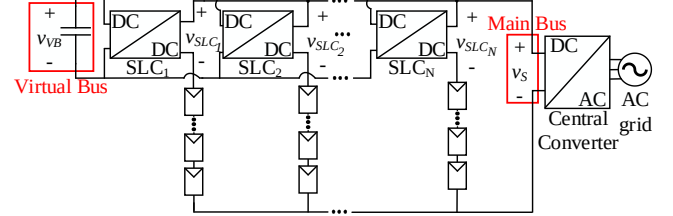
Fig. 2. PV systems using proposed PV2VB PDPP.
