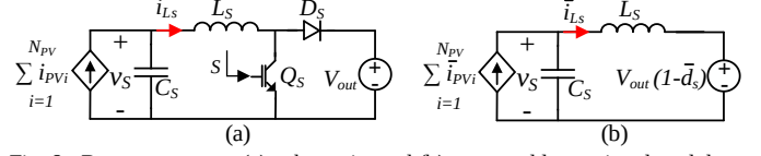
Fig. 8. Boost converter: (a) schematic, and (b) averaged large signal model. switching cycle, we can successfully derive the boost converter equations for the state-space model:
