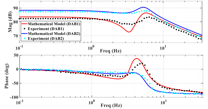
Fig. 14. The \Phi_i(s) to V_{IB_i}(s) transfer functions. The input used for system identification is a two-period 11-bit PRBS with clock frequency of 100 Hz.
