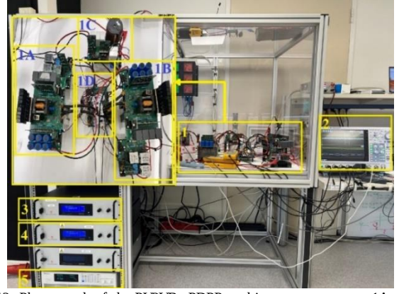
Fig. 12. Photograph of the PV2VB PDPP architecture prototype. 1A: SLC 1 , 1B: SLC 2 , 1C: Central converter, 1D: Micro controller, 2: YOKOGAWA DLM5038 oscilloscope, 3 and 4: SM1500-CP-30 Bi-directional DC Power Supplies, 5: 6210H-600S Programmable DC Power Supply.
