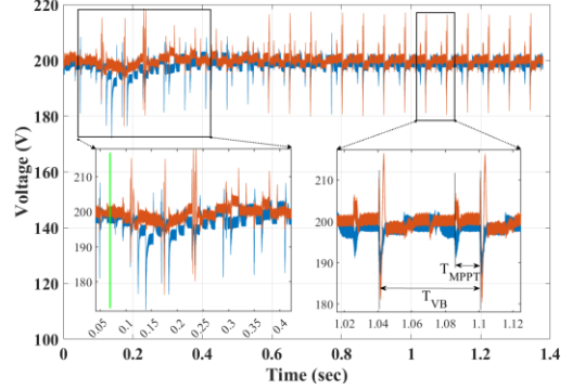
Fig. 20. Transition of intermediate bus voltages in the PV2VB PDPP architecture (blue: V_{IB1} , red: V_{IB2} ).
