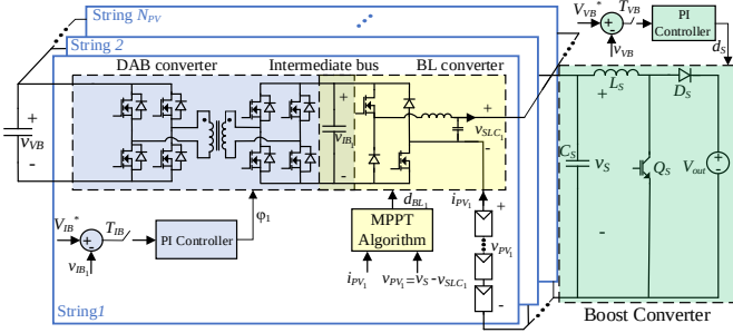
Fig. 15. PV2VB PDPP architecture with its control loop block diagrams. efficient operation. Considering a search-based MPPT algorithm like P&O, the system inherently has two categories of feedback (error-based) control loops: one central converter controller and N_{PV} DAB converter controllers (Fig. 15).
