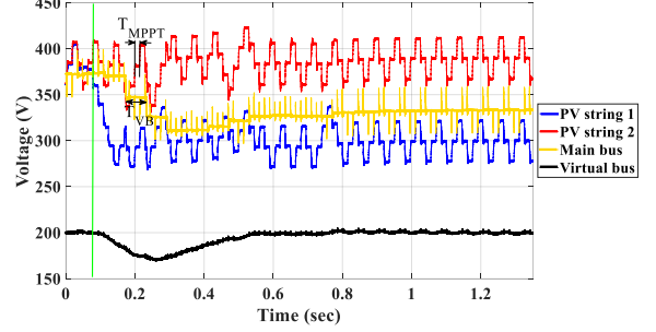
Fig. 19. Voltage waveforms in the PV2VB PDPP architecture. PV string 2 stays at I-V curve 1, whereas PV string 1 transitions from I-V curve 1 to I-V curve 2 after 0.07 s, highlighted with the green line.
