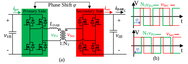
Fig. 5. DAB Converter. (a) Topology. (b) Waveforms using SPS modulation. Top: the primary side leads the secondary side, and the energy is transferred from the virtual bus to the intermediate bus. Bottom: the secondary side leads the primary side, and the energy transfer direction is reversed.
