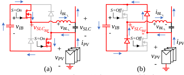
Fig. 6. BL converter operation during (a) the ON-state and (b) the OFF-state.
