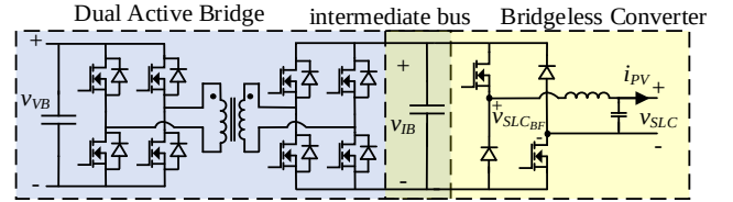
Fig. 3. Proposed SLCs topology for PV2VB PDPP architecture: A DAB converter followed by a BL converter.
