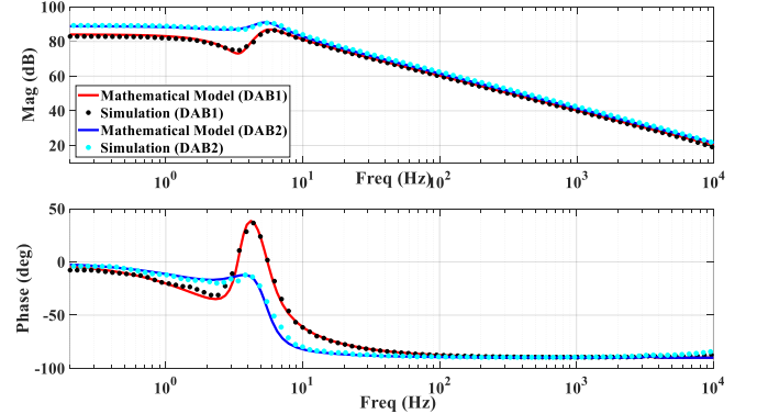
Fig. 11. \Phi_i(s) to V_{B_i}(s) transfer functions. The input used for system identification is a two-period 17-bit PRBS with clock frequency of 50 kHz.
