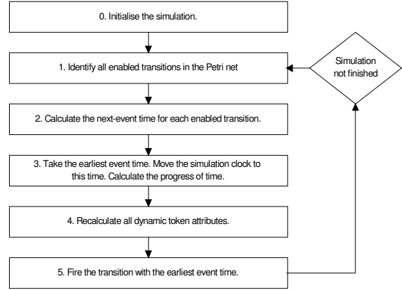
Figure 7: Simulation logic
