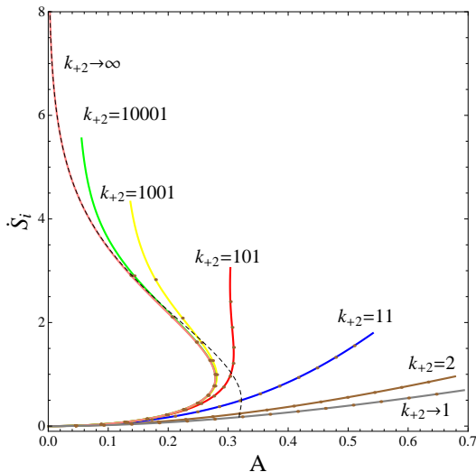
FIG. 4: (Color online) Same type of plot as Fig. 1 but for entropy production.
