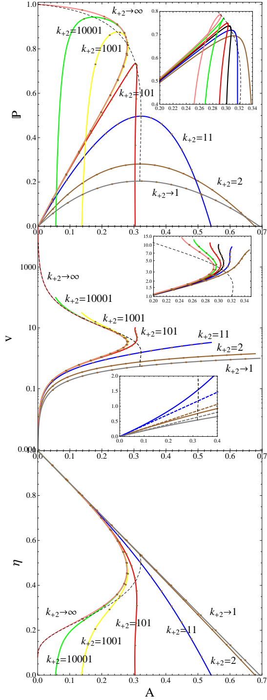
FIG. 1: (Color online) The full thick curves represent the parametric dependence on 0 \leq \epsilon \leq \ln 2 of the power \mathbb{P} , the copolymerization speed v , and the efficiency \eta on the ordinate and the affinity A as abscissa. The point \epsilon = \ln 2 is located at the origin of the axes for \mathbb{P} and v and at \eta = 1 and A = 0 for \eta . The small dots along the curves are separated by \Delta\epsilon = (\ln 2)/14 to indicate how fast \epsilon changes along the curves. Different thick curves correspond to different choices of k_{+2} , with k_{+1} \leq k_{+2} \leq \infty . Without loss of generality we set k_{+1} = 1 (time rescaling). The thin dashed curves intersect the thick curves where the value of \epsilon corresponds to maximum power with respect to \epsilon . The curves in the inset in the \mathbb{P} plot and in the upper inset of the v plot correspond to k_{+2} = 65, 85, 105, 121, 160, and 200 . The dashed curves in the lower inset of this plot represent the linear response predictions v = LA for k_{+2} = 1, 2, 11 .
