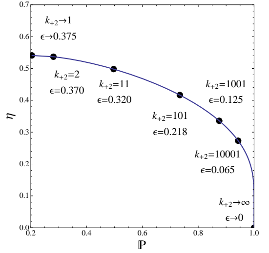
FIG. 2: (Color online) Efficiency \eta and power \mathbb{P} corresponding to the maximum power denoted simply by \epsilon in the figure for different values of k_{+2} . We have set k_{+1} = 1 .
