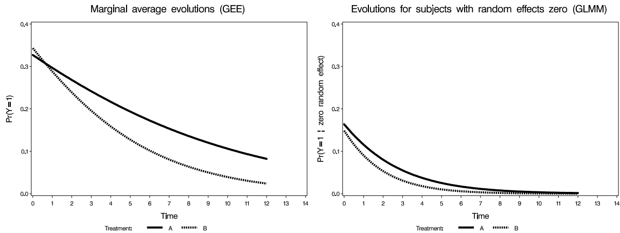
Figure 6: Toenail Data . Treatment-specific evolutions . (a) Marginal evolutions as obtained from the marginal model (3.6) fitted using GEE , (b) Evolutions for subjects with random effects in model (3.7) equal to zero .
