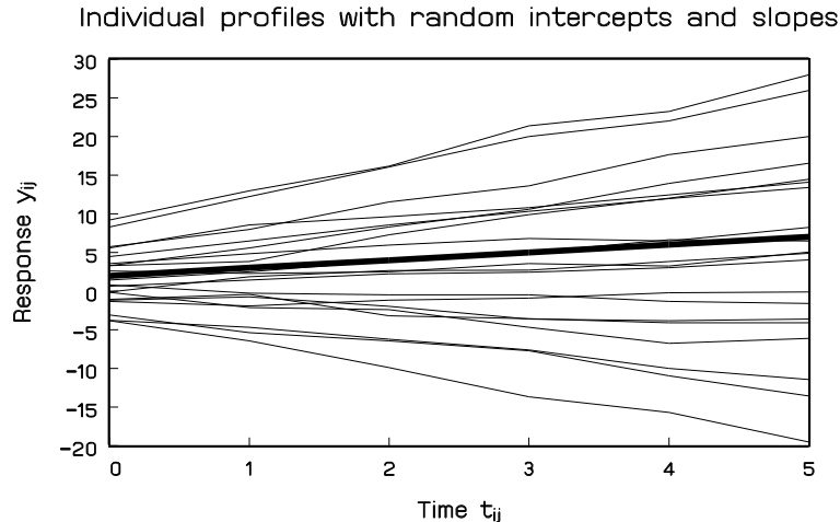
Figure 3: Hypothetical example of continuous longitudinal data which can be well described by a linear mixed model with random intercepts and random slopes. The thin lines represent the observed subject-specific evolutions. The bold line represents the population-averaged evolution. Measurements are taken at six time-points 0, 1, 2, 3, 4, 5.
