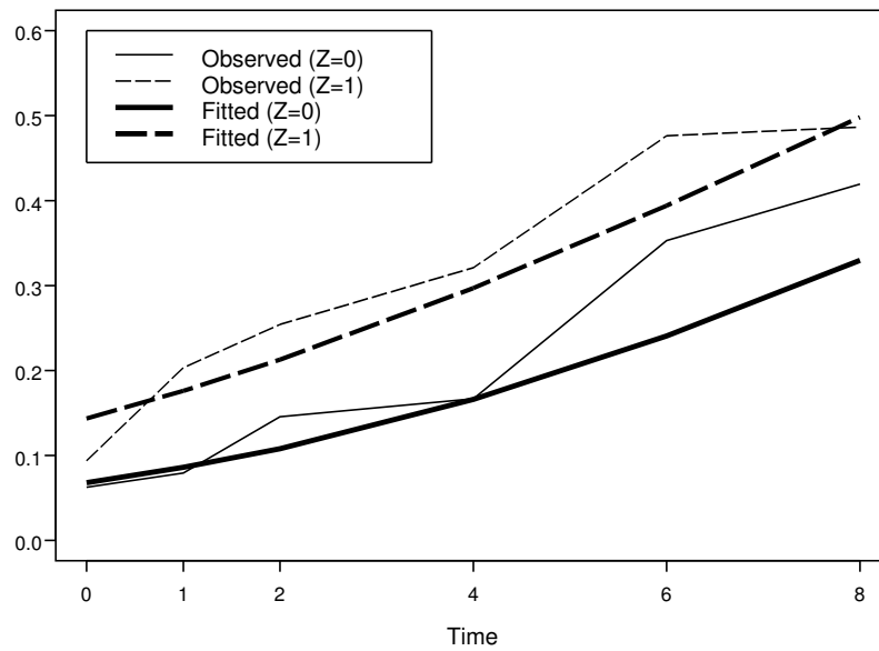
Figure 1. Evolution of the observed and fitted (using Model (1)) probabilities to be classified as a normal to mildly ill patient by treatment group. Here Z = 1 ( 0 ) denotes the treatment (control) group.
