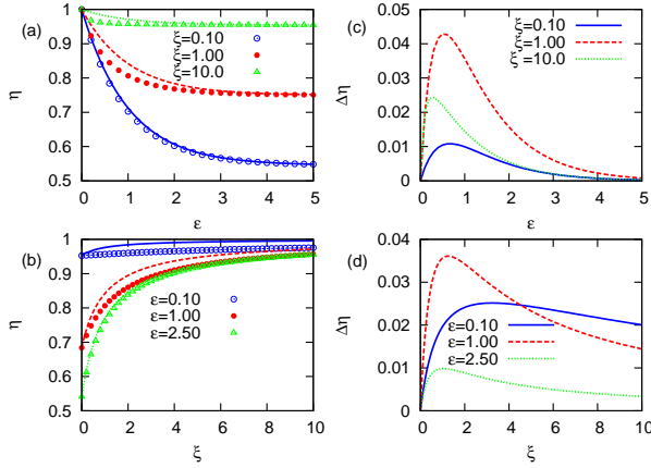
FIG. 3. (Color online) (a) Efficiency \eta as a function of \epsilon for different values of \xi . The lines are for a classical bath and the symbols for a quantum bath. (b) \eta versus \xi for different values of \epsilon . The lines are for a classical heat bath and the symbols for a quantum bath. (c) Difference of efficiencies between the classical and quantum bath cases as a function of \epsilon for various values of \xi . (d) Difference of efficiency between the classical and quantum bath cases as a function of \xi for various values of \epsilon .
