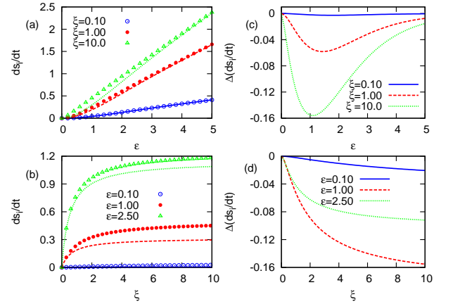
FIG. 2. (Color online) (a) Entropy production rate \dot{s}_i as a function of \varepsilon for different values of \xi . The lines are for a classical bath and the symbols for a quantum bath. (b) \dot{s}_i versus \xi for various values of \varepsilon . The lines are for a classical bath and the symbols for a quantum bath. (c) Difference in entropy production rates between the classical and quantum bath cases as a function of \varepsilon for various values of \xi . (d) Difference in entropy production rates between the classical and quantum bath cases as a function of \xi for various values of \varepsilon .
