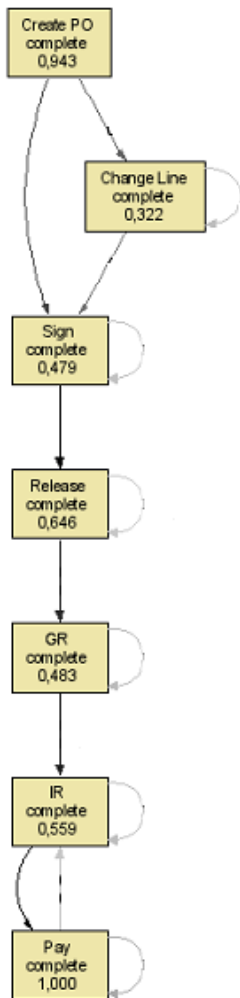
Figure 2. Output of Fuzzy Miner with default settings to uncover the core process in the event log.
