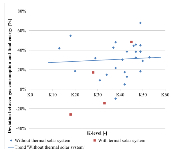
Figure 9 Mean deviation between measured gas consumption and calculated final energy for heating and hot water as a function of K-level and the presence of a thermal solar system. (positive deviation: calculation overestimates real consumption, negative deviation: calculation underestimates real consumption)
