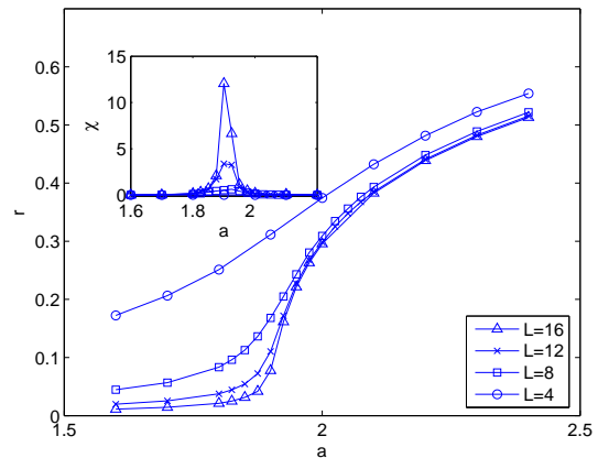
FIG. 12: Transition in d = 4 : The behavior of the order parameter near the transition point is shown for various system sizes. The inset shows the generalized susceptibility, \chi , which peaks at a = 1.900 \pm 0.025 , giving an estimation of a_c .
