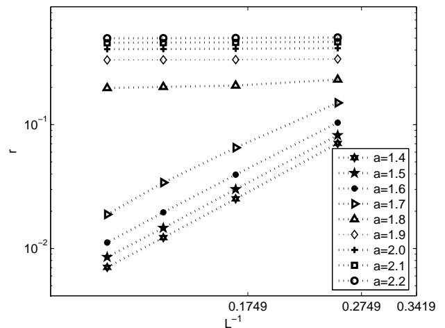
FIG. 16: Log-log plots of r vs L^{-1} in d = 5 . The order parameter r clearly approaches a finite, nonzero value for a > a_c and approaches 0 for a < a_c . The value of a_c appears to fall between a = 1.8 and a = 1.7 .
