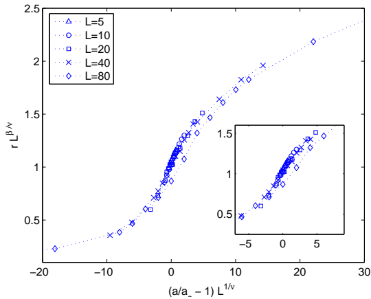
FIG. 10: Exponents in d = 3 . Data collapse of rL^{\frac{\beta}{\nu}} vs (a/a_c - 1)L^{\frac{1}{\nu}} . With a_c = 2.345 , we show the data collapse using theoretical Ising 3D exponents. The collapse is reasonable good, but still poor compared with that seen with exponents from the XY class. Insets show a closer view near the critical point.
