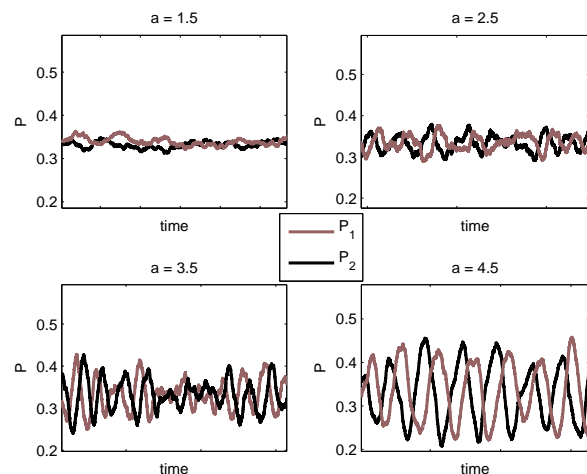
FIG. 3: Absence of synchronization in 2D. Top left: a = 1.5 . Top right: a = 2.5 . Bottom left: a = 3.5 . Bottom right: a = 4.5 . L = 100 for all plots. Even for very large values of the coupling, highly synchronous oscillatory behavior is not present. As discussed in the text and shown in the next figure, the intermittent oscillations apparent for high values of a result from finite size effects.
