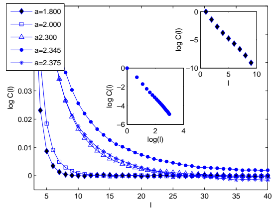
FIG. 11: Spatial correlations in d = 3 . As a approaches the critical value a_c , evidence of long range correlations develops, indicative of a diverging correlation length at the critical point. The lower inset shows the power law decay of the correlation function at the critical point, while the upper inset shows that the correlation function decays exponentially far from the critical point.
