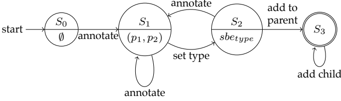
Figure 7.2: An annotation is ready when the annotation is drawn and a storyboard element type is set
