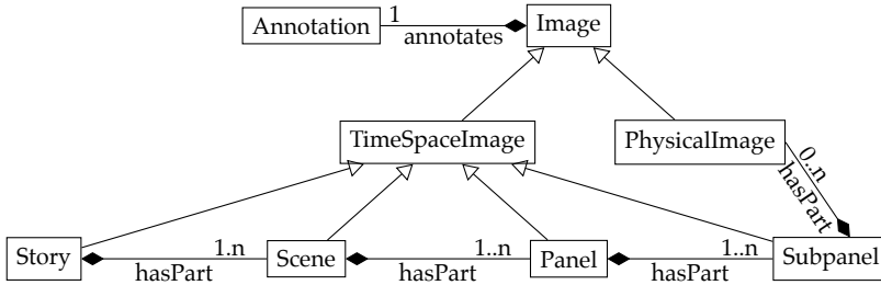
Figure 5.2: A storyboard contains images to visualize the passage of time as well as physical items. The passage of time is visualized by the structure of the storyboard and the size of images
