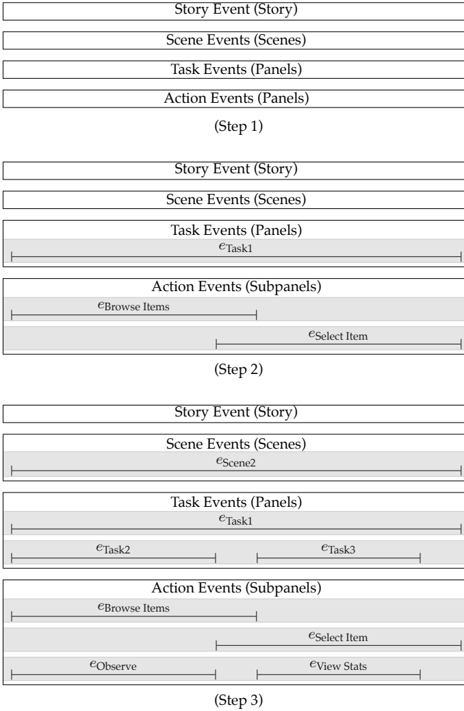
Figure 6.3: State of the array levels (white boxes) as createTimeline traverses the events hierarchy in Figure 6.2 to generate a timeline of the storyboard in Figure 5.5. Grey lanes contain events. Two or more lanes in one level are added to avoid placing events that intersect in time on top of each other. Step 3 shows the events for the timeline in Figure 6.1
