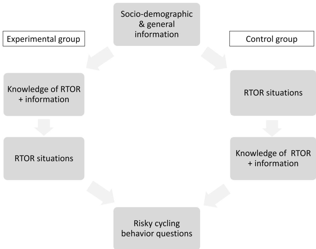
FIGURE 2 Survey structure.
