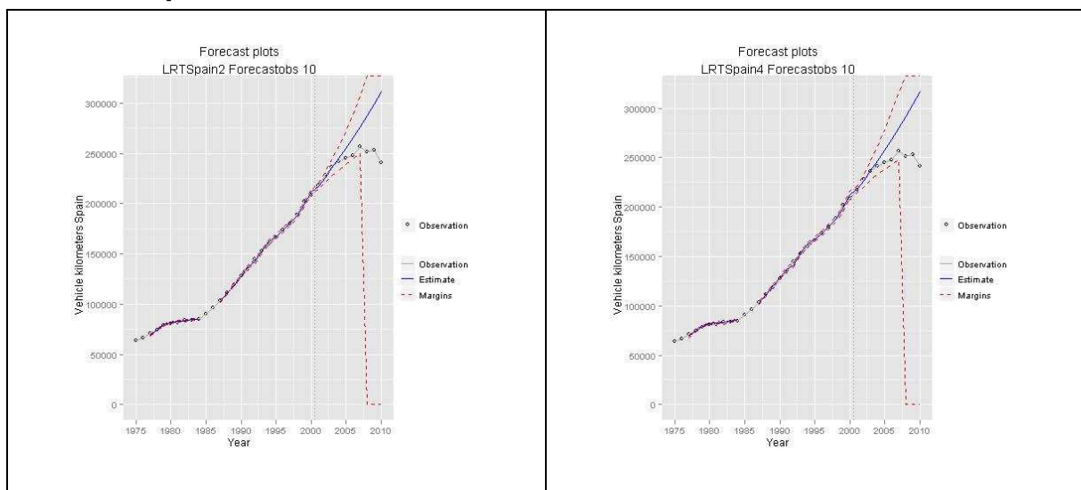
Figure 6: Plots comparing the model predictions (straight line) with the actual observations
