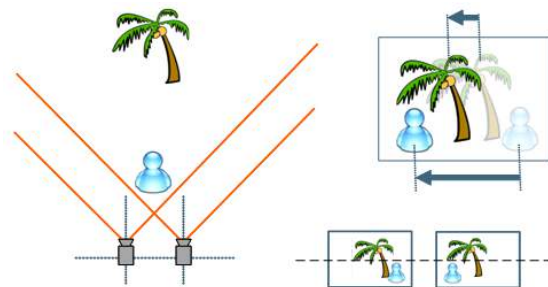
Figure 1: Concept of stereo vision. A scene is captured using 2 rectified cameras. Stereo matching attempts to estimate the apparent movement of the objects across the images. A large apparent movement (i.e. parallax) corresponds to close objects (a low depth value) and vice versa.
