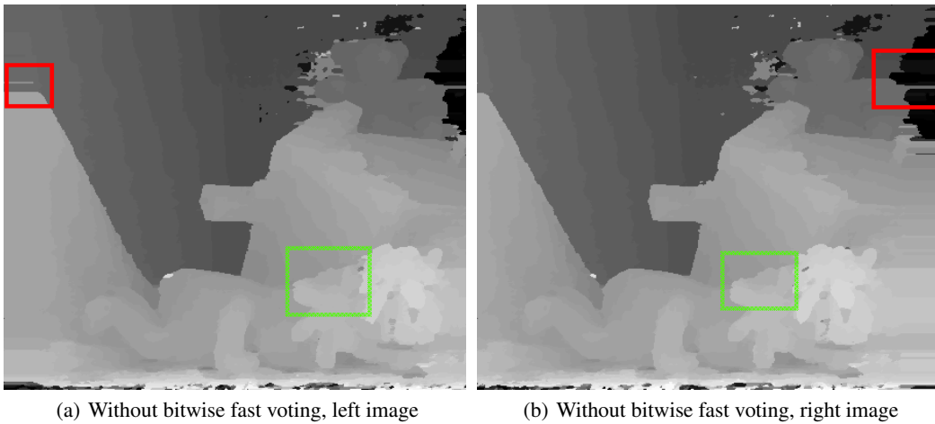
Figure 6: Results without bitwise voting. The results with bitwise voting are shown in Figure 5, (a) and (c). The red, full squares show the result at the borders of the disparity maps. Not enough information is available in both images to estimate the disparity correctly. Therefore, filling these values naively will result in erroneous lines. By using bitwise voting, these artifacts are eliminated. The green, dashed squares show the handling of invalid disparity values around edges in the images (i.e. occlusion). When no bitwise voting is applied, edges are fattened and the disparity values leak over the edges, resulting in artifacts. This is avoided by incorporating color information.
