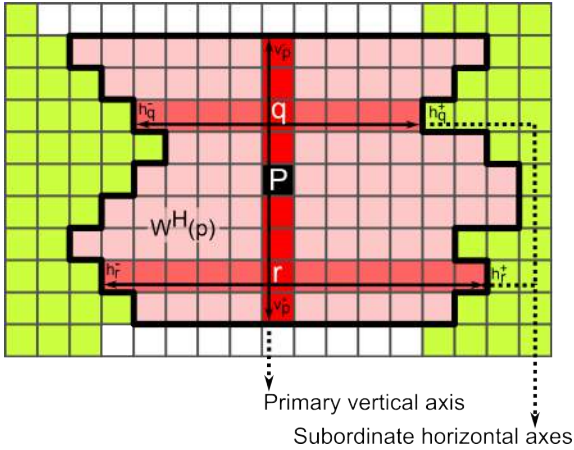
Figure 2: Derivation of the horizontal support window W^H using each pixel's axis-defining quadruple (h_p^-, h_p^+, v_p^-, v_p^+) .
