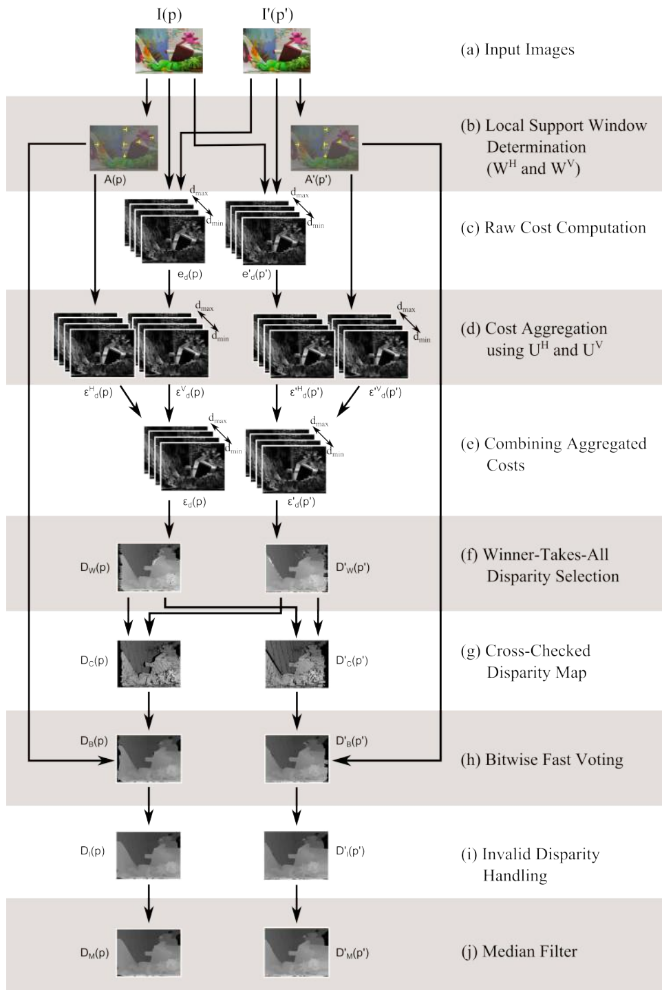
Figure 4: Overview of our method. (a) The input is a pair of rectified stereo images, in our case the standard Middlebury dataset Teddy (Scharstein and Szeliski, 2003) (b) First, we calculate the local support windows, based on color similarities in each image. (c) Next, we calculate the pixelwise cost per disparity. (d) These costs are aggregated, based on the support windows. There are 2 windows, and therefore 2 sets of aggregated costs. (e) The costs of the 2 windows are combined. (f) Next, we select the most suitable disparity value using a Winner-Takes-All approach. (g) A cross-check is performed to find any mismatches, typically caused by occlusions around edges. (h) The local support windows are used again to determine the most occurring disparity value in each window. This increases the quality of the disparity map. (i) Finally, any remaining invalid disparities are handled and (j) a median filter is applied to remove noise. The result is 2 disparity maps, one for each input image.
