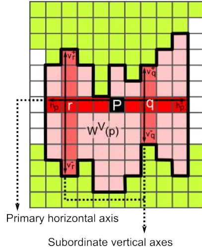
Figure 3: Derivation of the vertical support window W^V using each pixel's axis-defining quadruple (h_p^-, h_p^+, v_p^-, v_p^+) .
