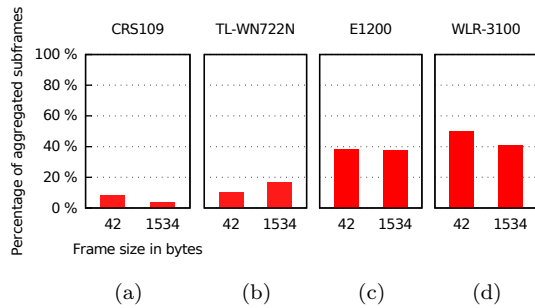
Figure 5: The percentage of aggregated subframes received per 250,000 transmitted frames from attacker to victim in our test setup shows that except for the TL-WN722N ( hostapd ) device, using small frames results in a slightly higher aggregation rate.
