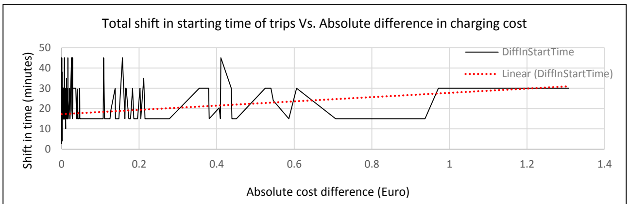
Figure 6 Comparison between total absolute shift in trips and absolute difference in total charging cost
