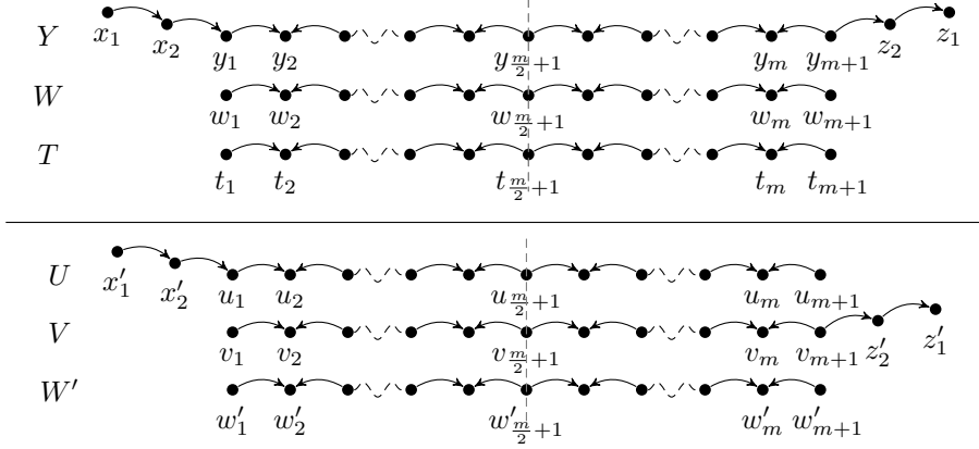
Figure 2: Graphs G_1^m (top) and G_2^m (bottom) used to establish boolean separation in the proof of Proposition 5.4.
