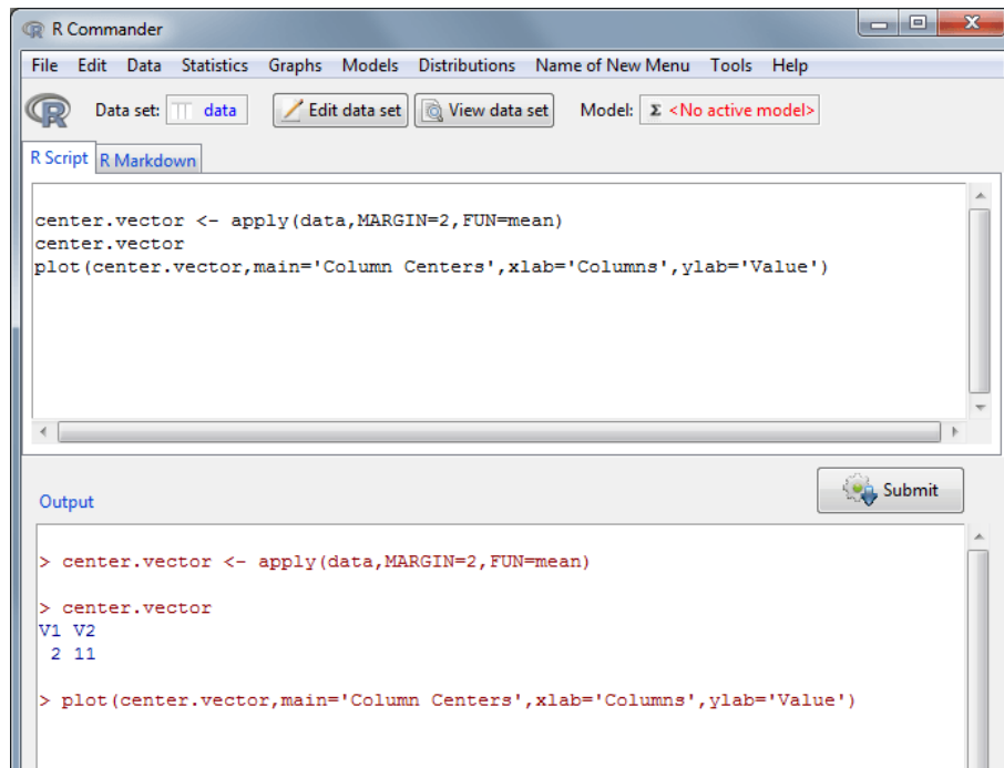
Figure 17: Example - CenterColumns
