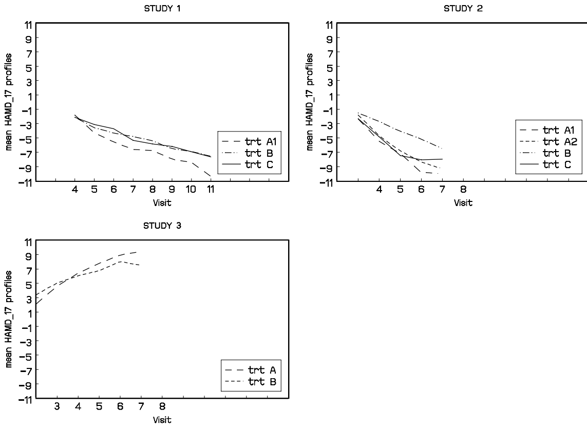
Figure 1: Mean profiles for each of the three studies.
