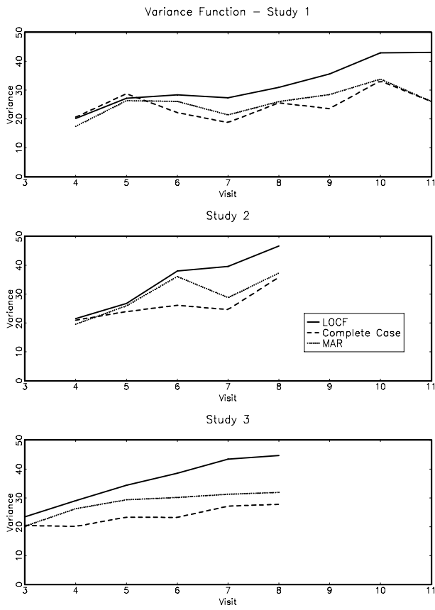
Figure 4: Variance Functions per Study and Per Method.
