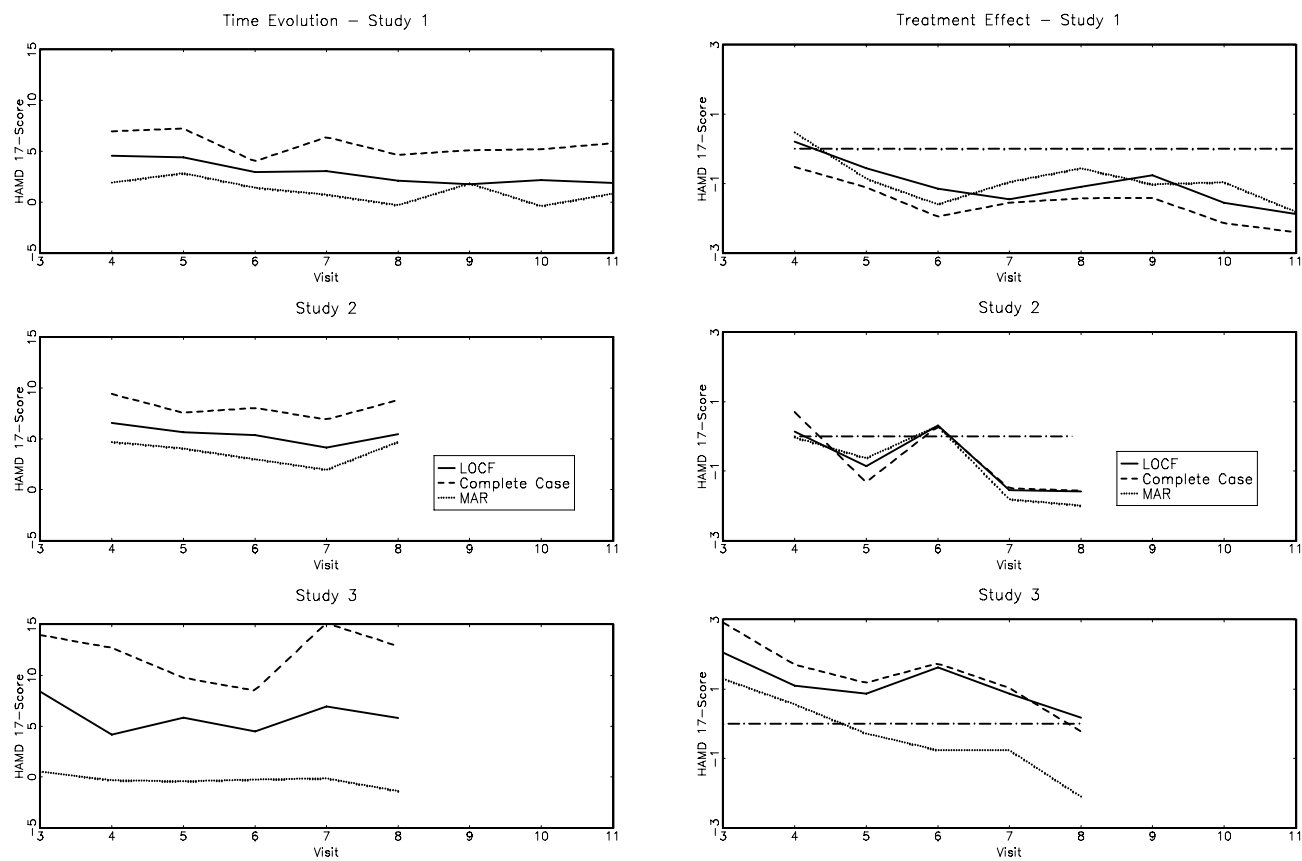
Figure 3: Summary of All Placebo Time Evolutions (left hand panels) and All Treatment Effects (right hand panels).
