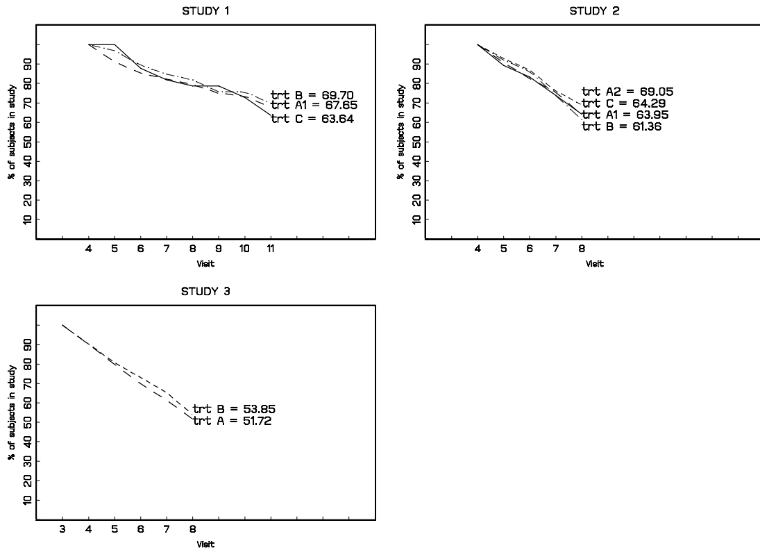
Figure 2: Evolution of dropout per study and per treatment arm. Treatment arms of primary interest, are shown in bolder typeface.
