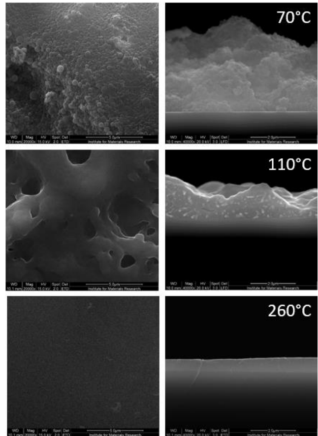
Figure 4 SEM images of layers during the annealing process. (Left) Top-view; scale bar is 5 \mu\text{m} (Right) cross-section; scale bar is 2 \mu\text{m} .
