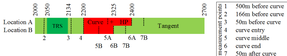
(e) FIGURE 1 (a) Curve properties; real world vs. simulator images nearby curve entry at (b) location A and (c) location B; (d) simulator image of TRS (left) and HP (right); (e) scenario overview
