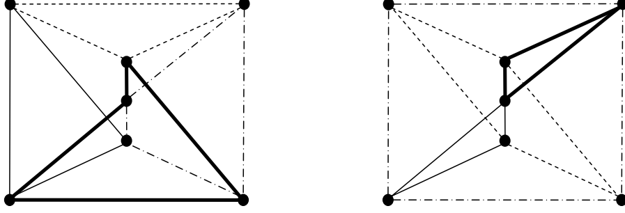
Figure 16: Two circuit partitions in a graph of crossing number 2.
