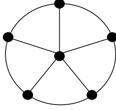
Figure 3: The wheel graph W_5 .
