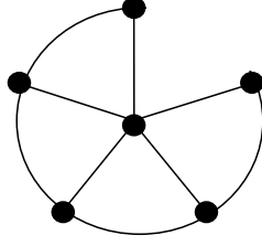
Figure 2: A graph locally equivalent to a bipartite graph.
