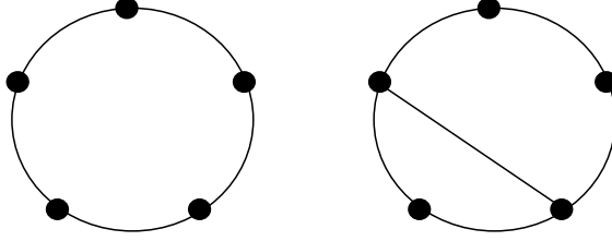
Figure 1: C_5 and H .
