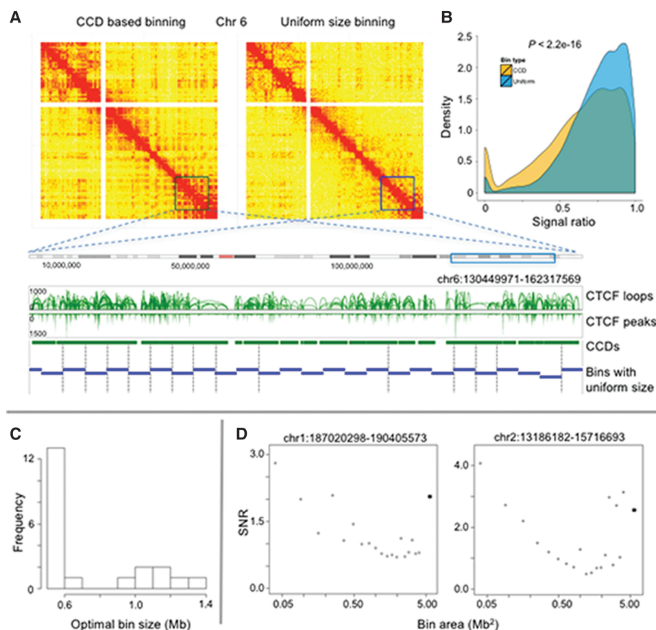
Figure 3. Comparison of data-driven vs. uniform size genomic binning procedure. (A) Contact maps were generated using CCD-based binning (left) and uniform size binning (right) for Chromosome 6, respectively. The sizes of tiles in the contact map correspond to their genomic lengths. The same color scale was used for both contact maps. The squares in the contact maps were enlarged as a zoomed-in region, shown below in a genomic browser track view, in which the CCD-based bins are in green and the uniform-sized bins are in blue. The vertical dashed lines indicate the split of functional CCDs into pieces by uniform-sized bins. (B) Distribution of interaction frequency ratio for neighboring bins for all chromosomes by CCD (yellow) and uniform (blue) bins. (C) Histogram of the optimal bin size for 21 long-range interactions identified in the ChIA-PET library. (D) Plots of the SNR as a function of uniform bin area for two of the long-range interactions. The values for the CCD-based bins are indicated by dark squares. The chromosome coordinates of each interaction are listed above the plots.
