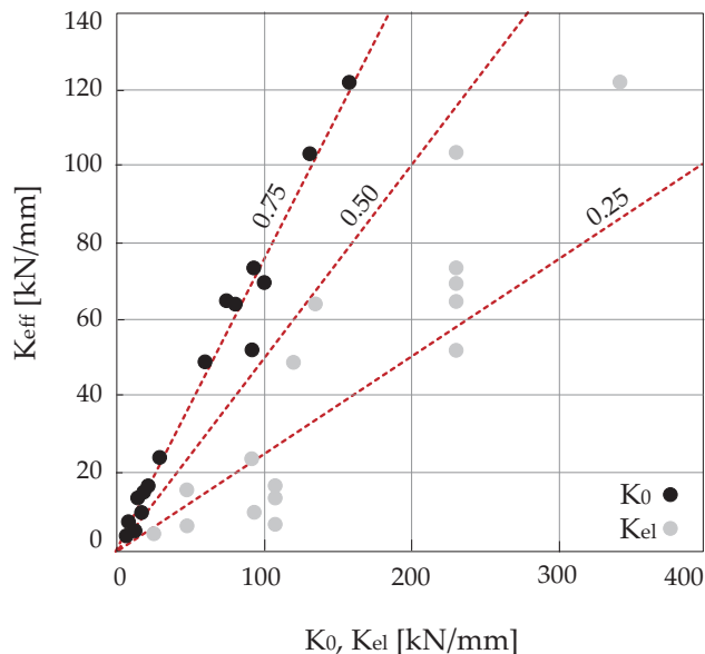
Figure 1. Stiffness comparisons.
