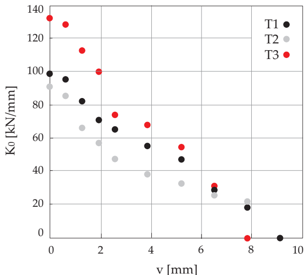
Figure 2. Stiffness degradation.
