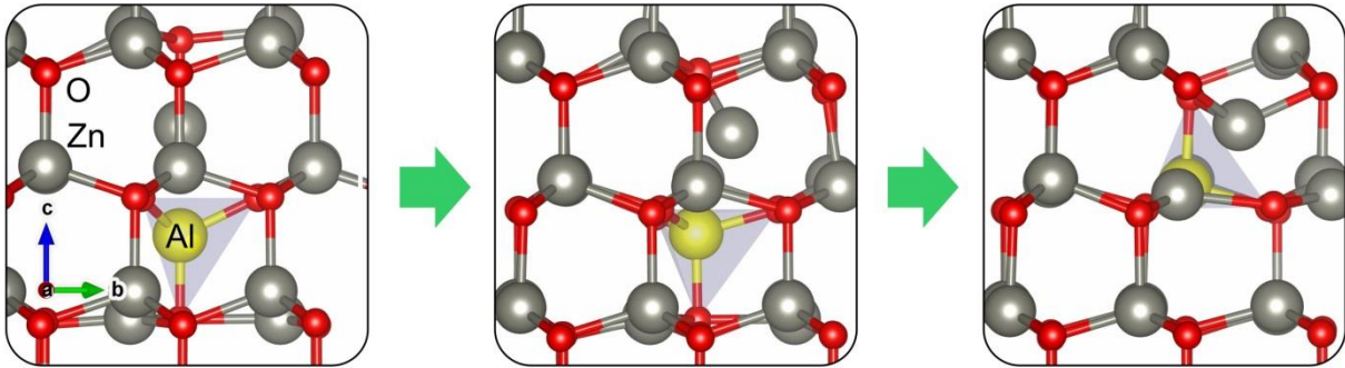
Figure 8. The structural transition from the relaxed Al defect towards the Al_{Zn}-Zn_i complex, all in the 1+ charge state.
