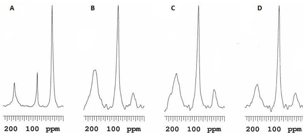
Figure 12. NMR spectra of AZO: a) as-synthesized, b) after 10min annealing, c) 30min annealing, d) 2 hour annealing.
