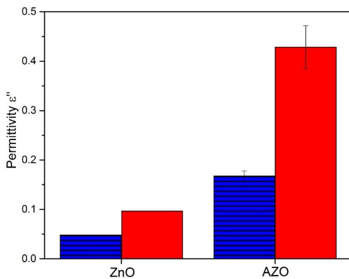
Figure 3. MCPT measurements result at 2.4GHz. Blue (horizontal lines) - as-synthesized, red (empty) – annealed, with standard deviation bars.
