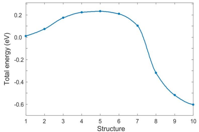
Figure 11. Barrier energy between Al_{Zn}-Zn_i (D1) complex and the Al_{Zn}-Zn_i (D2) complex in ZnO, system in the 1+ charge state.
