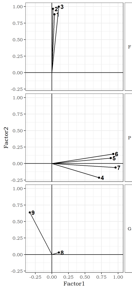
Figure 6: Factor loadings for a factor analysis with 3 factors and promax rotation.
