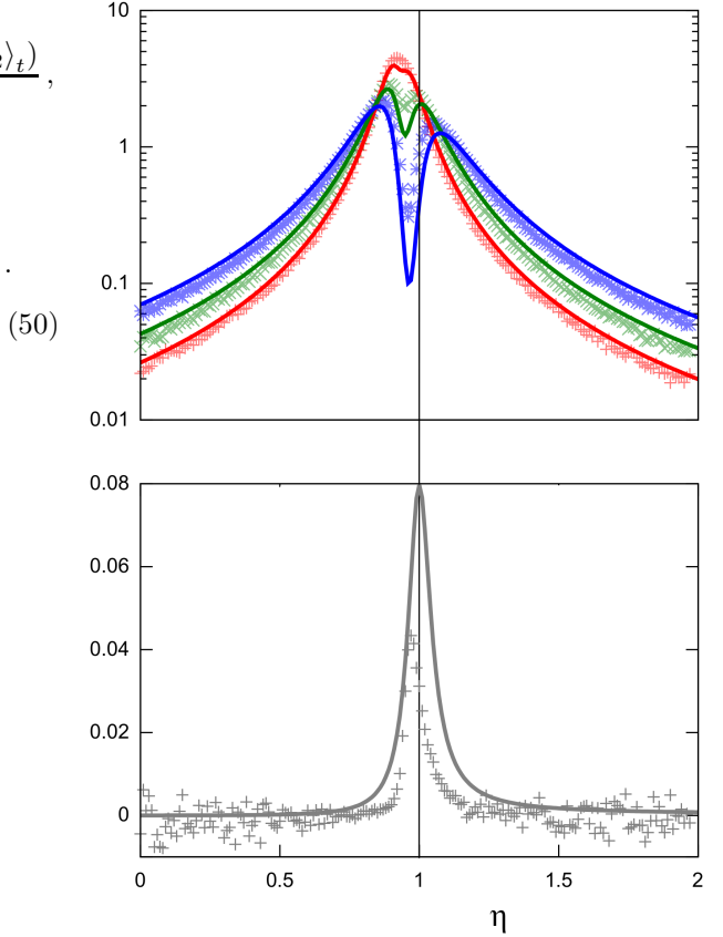
FIG. 4. Stochastic efficiency of a Brownian duet with time-symmetric driving: g_1(t) = 10 \cos(2\pi t/\tau) and g_2(t) = 10 \cos(2\pi t/\tau) + \cos(4\pi t/\tau) with thermodynamic forces X_1 = -X_2 = 10 , which leads to \bar{\eta} = 0 . Upper panel: probability distribution of the efficiency after 32 (red), 64 (green) and 128 (blue) cycles with analytical results and simulation data. Lower panel: Large deviation function of the efficiency, with analytical results and extrapolation from simulation data (using the extrapolation procedure described in [53, 55]).
