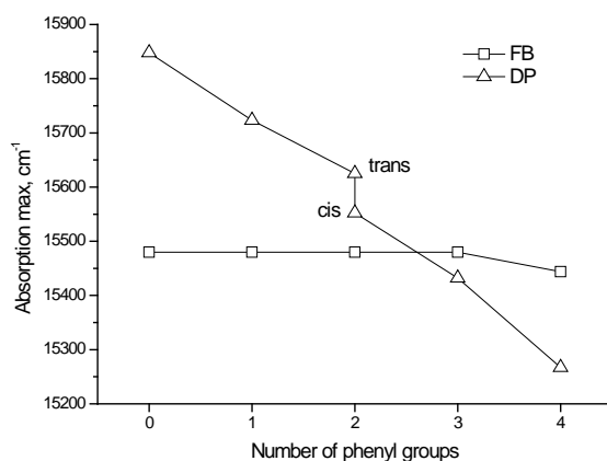
Figure 3. Absorption maximum as a function of the number of phenyl groups attached for the FB and DP forms
