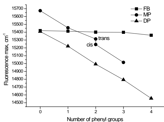
Figure 5. Fluorescence maximum as a function of the number of phenyl groups attached for the FB, MP and DP forms
