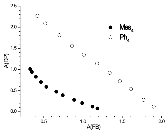
Figure 2. Relationship between the absorptivities measured at the maxima of the Soret bands for the FB and DP forms during the course of the titration for Mes 4 (●) and Ph 4 (○)
