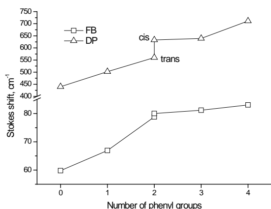
Figure 6. Stokes shift as a function of the number of phenyl groups attached for the FB and DP forms
