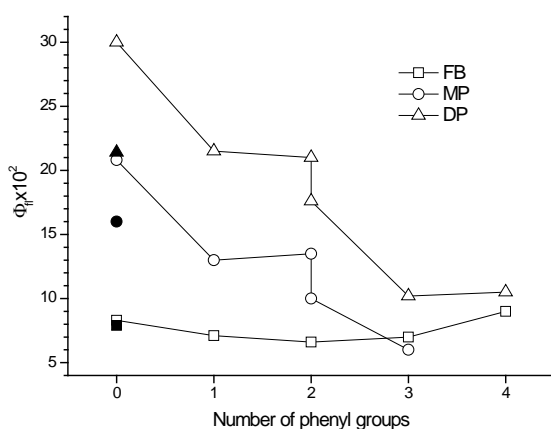
Figure 7. Fluorescence quantum yield as a function of the number of phenyl groups attached for the FB, MP and DP forms. The closed symbols indicate the corresponding data for the three species of Mes 4 measured in THF-TFA solutions [28]
