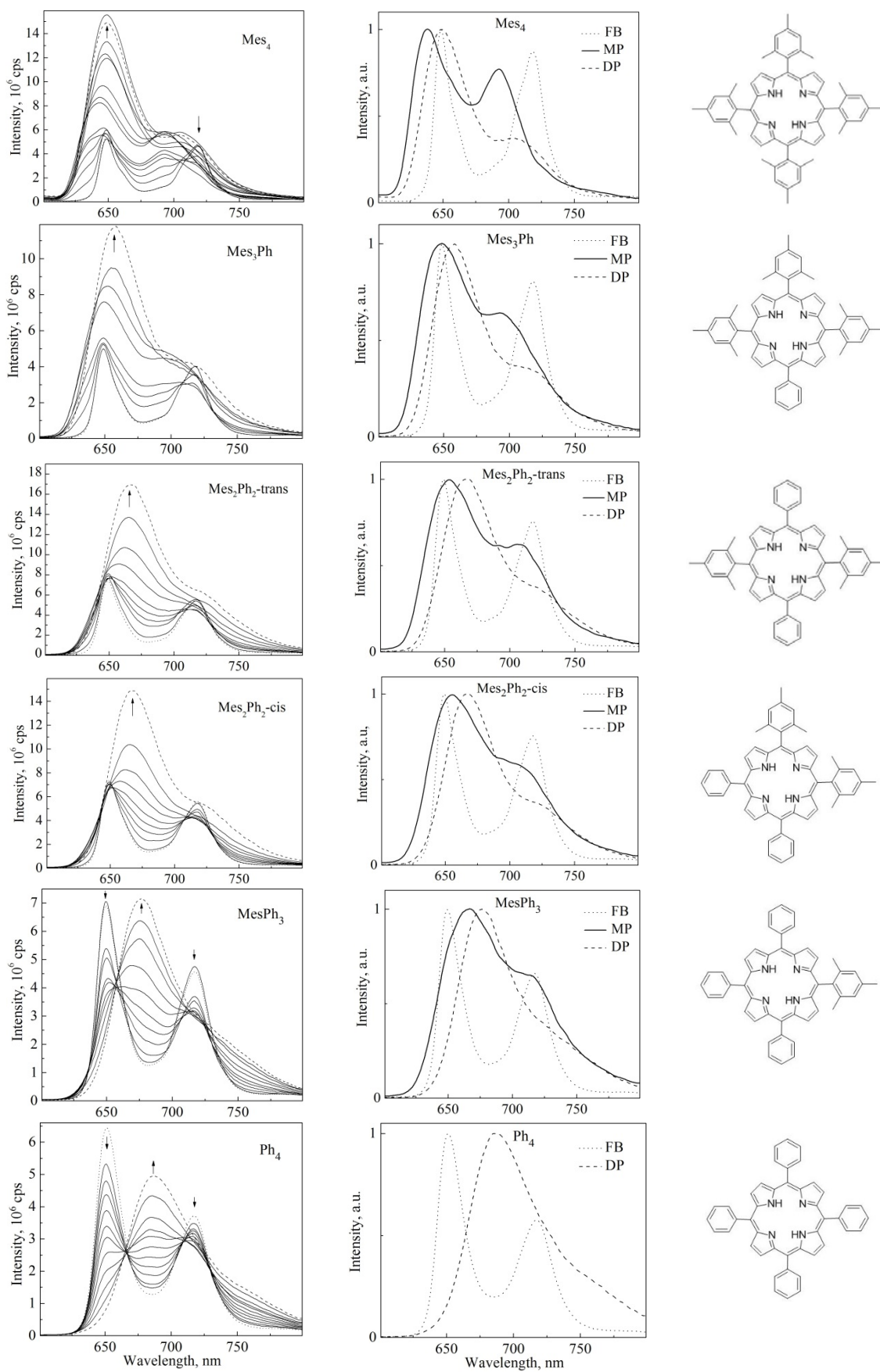
Figure 4. Absorbance-normalized fluorescence spectra measured during the course of the titration (left), individual (normalized) fluorescence spectra of the FB, MP and DP forms (center), and molecular structures of the corresponding tetraarylporphyrins (right)
