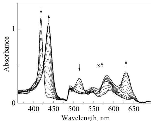
Figure 1. Ground state absorption spectra of Mes 4 measured during the course of the titration. The arrows indicate the direction of the spectral changes upon going from the FB to the MP and DP forms
