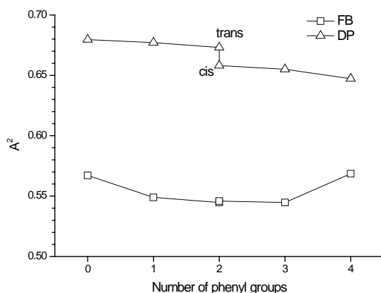
Figure 8. Weight A^2 of the one electron ( a_{2u}, e_g ) configuration as a function of the number of phenyl groups attached for the FB and DP forms
