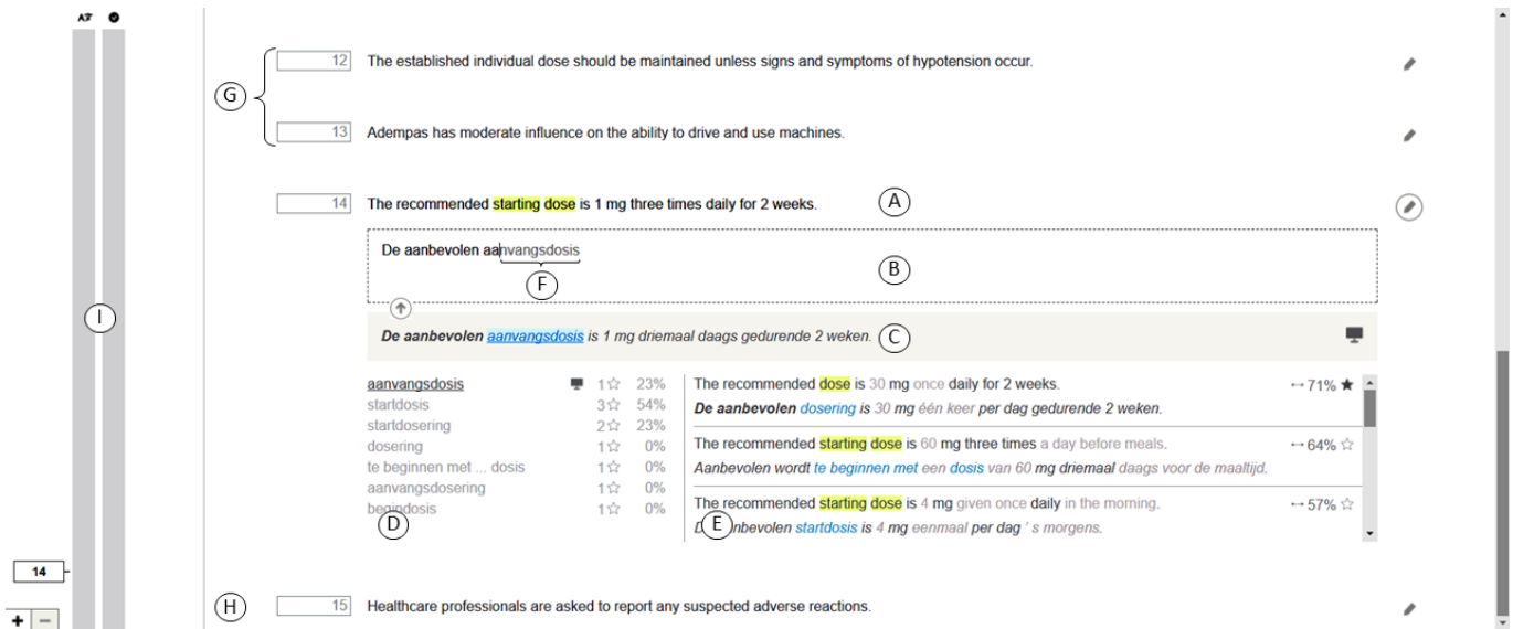
Figure 1. An overview of the Intellingo user interface when translating: A the source segment, B a text area for the user translation, C machine translation, D alternative word groups, E related earlier translations (translation memory), F auto-completion, G two preceding segments, H the next segment and I a progress bar indication of translation and revision. Upon hovering over the translation suggestions, the related phrases are highlighted in yellow (source language) and blue (target language) across all suggestions.
