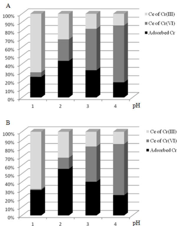
Fig. 2. Chromium distribution as a result of adsorption experiments on AC-dc-Mc (A) and AC-dc-Md (B) at different pH. Different colors of the columns represent adsorbed C_{r_{tot}} (black), C_e of Cr(III) in the solution (light grey) and C_e of Cr(VI) in the solution (dark grey). Experimental conditions: m = 0.030 \text{ g} , V = 50 \text{ ml} , C_o = 40 \text{ mg L}^{-1} , T = 25 \text{ }^\circ\text{C} , 48 \text{ h}
