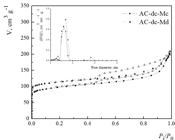
Fig. 1. N 2 adsorption isotherms of AC-dc-Mc and AC-dc-Md samples. Inset: Pore size distribution.
