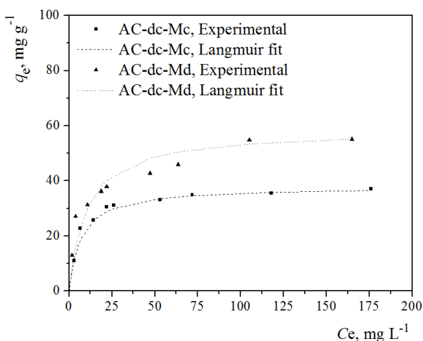
Fig. 4. Equilibrium Cr_{tot} adsorption isotherm for AC-dc-Mc and AC-dc-Md samples, i.e. experimental data and Langmuir fitting. Experimental conditions: initial Cr_{tot} solution pH = 2, m = 0.030 g, V = 50 ml, C_0 = 10-200 mg L -1 , T = 25 °C, 48 h.
