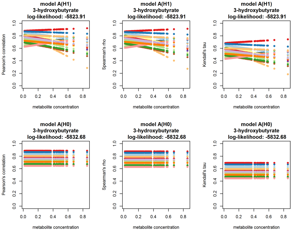
Figure 7.4: Estimated trajectories for the 3-hydroxybutyrate-co-expression association based on model A(H_1) and model A(H_0) in terms of Pearson's correlations, Spearman's rho, and Kendall's tau. The top row presents the results of the alternate model A(H_1) and the bottom row displays the results of the null-hypothesis model A(H_0) .
