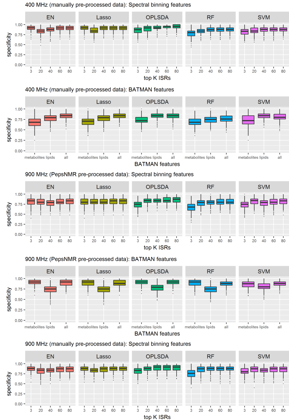
Figure 12.5: Box plots of the specificity of the elastic net, lasso, orthogonal partial least squares-discriminant analysis (OPLS-DA), random forest (RF), and support vector machine (SVM) classifiers.
