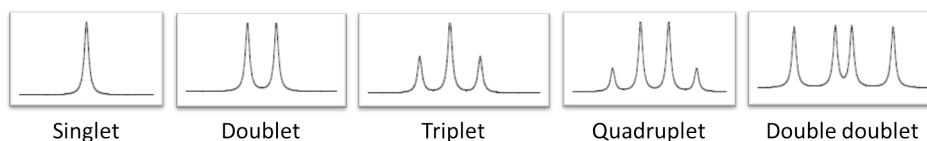
Figure 9.10: Examples of J-coupling patterns.
