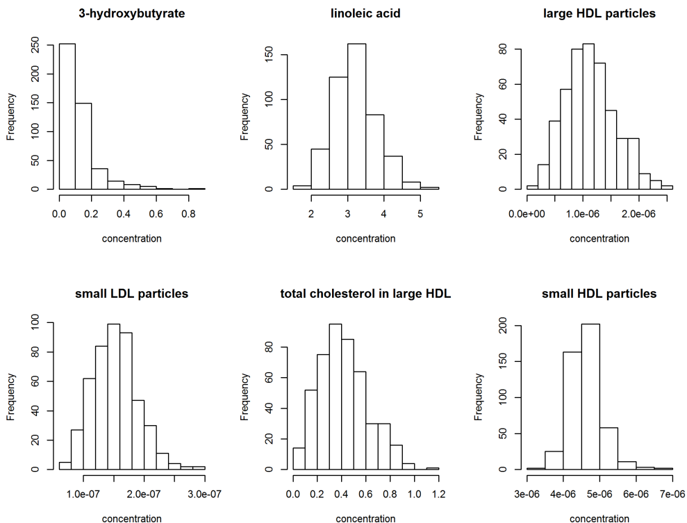
Figure 3.1: Histograms of the observed values for 3-hydroxybutyrate, linoleic acid, large HDL particles, small HDL particles, small LDL particles, and total cholesterol in large HDL.
