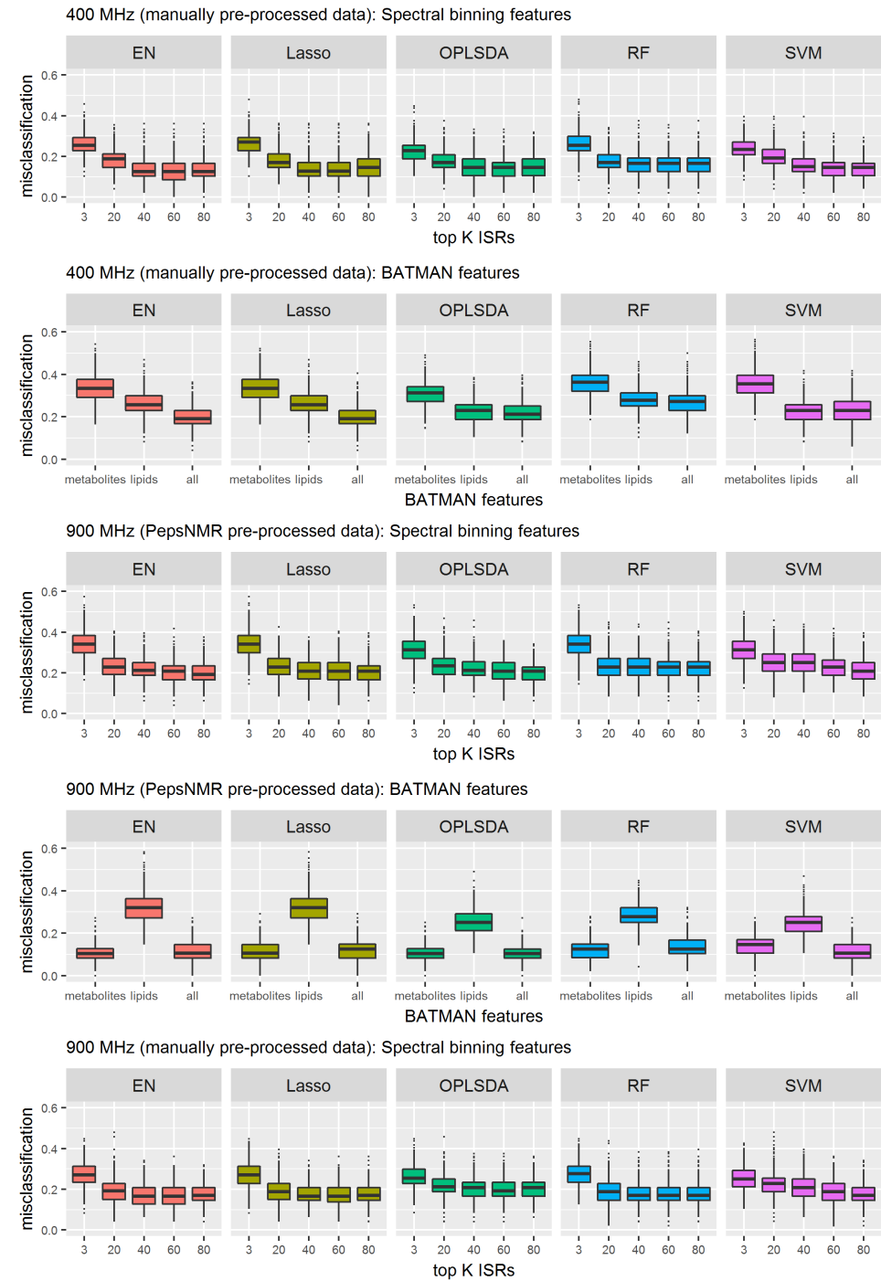
Figure 12.3: Box plots of the misclassification errors of the elastic net, lasso, orthogonal partial least squares-discriminant analysis (OPLS-DA), random forest (RF), and support vector machine (SVM) classifiers.
