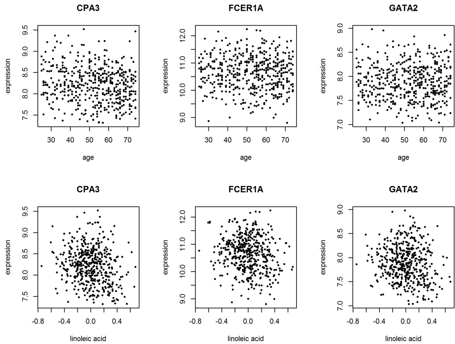
Figure A.1.2: Scatter plot of gene-expression values against age (top row) and gene-expression values against the concentration of linoleic acid (bottom row).
