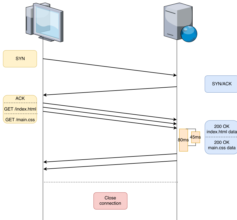
Figure 2.3: TCP connection that gets reused by the client, with pipelining. Index.html takes the server 80ms to process and main.css 45ms. However, the server needs to wait to send main.css until index.html has been sent.
