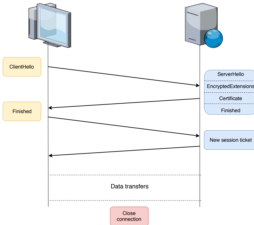
Figure 3.1: Handshake with QUIC which only takes one RTT for a secure connection
