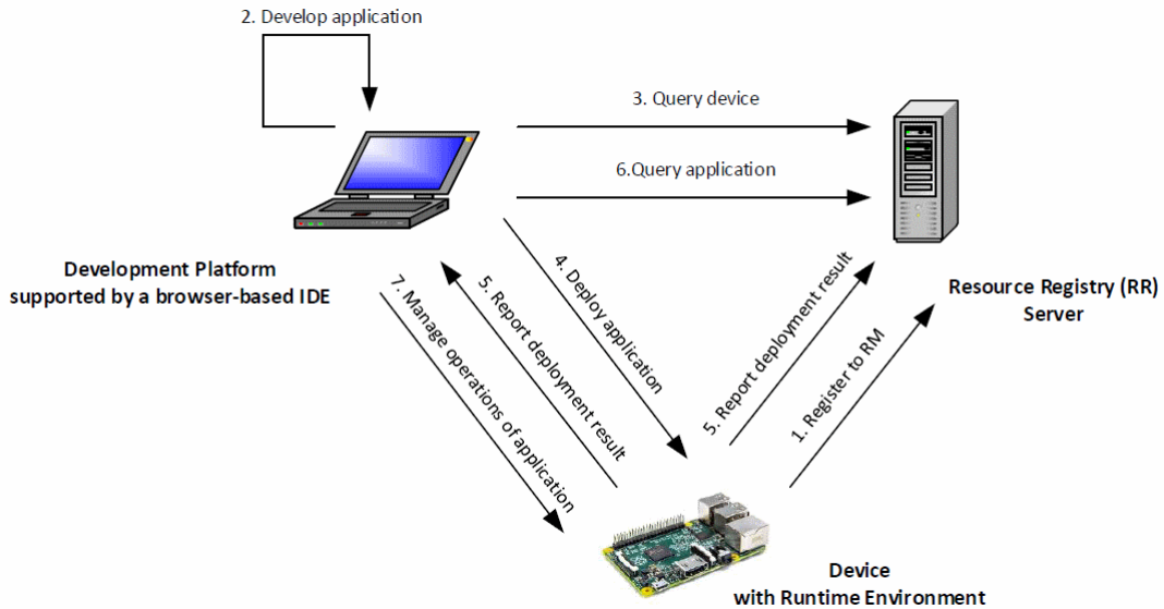
Figure 8: The flow of deploying and managing an application with LiquidIoT.
