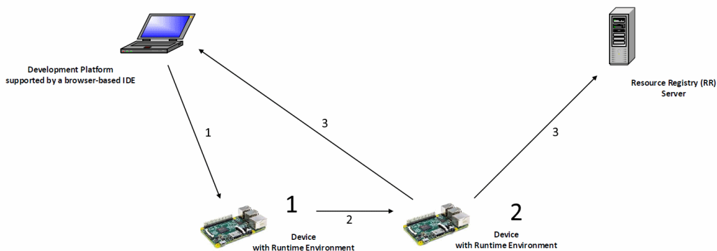
Figure 10: The source device packs a tarball that it can send to the target device.
