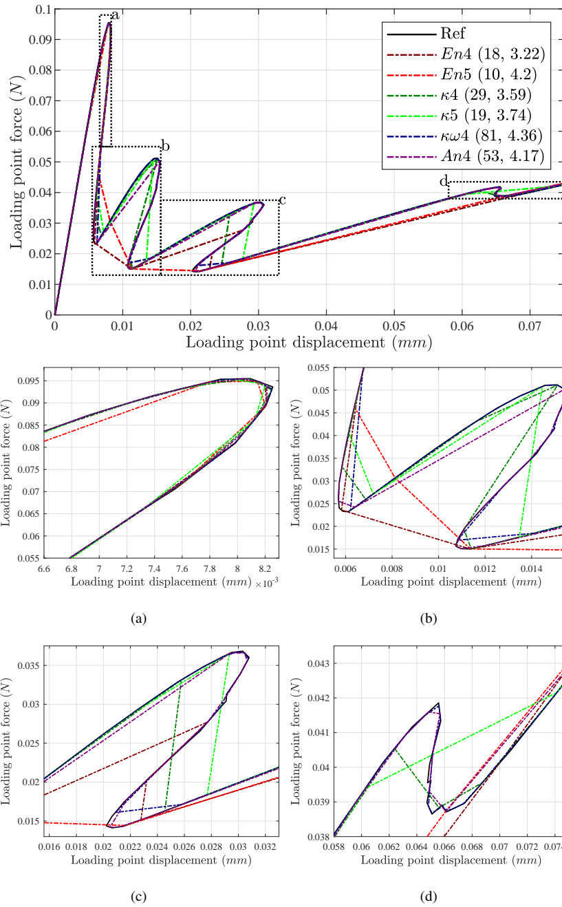
Figure 6: The presented constraints make the method proceed to the desired state although there are parts of the reference path which are skipped in the perforated beam problem. The black solid line represents the reference solution curve. the first number inside of the parentheses in front of the names of the constraint function shown in the legend indicates the total number of steps and the second one shows the average number of iterations per step. Zoom boxes 6(a) to 6(d) more clearly show the distance from the reference curve from the first to the fourth snap-back, respectively.
