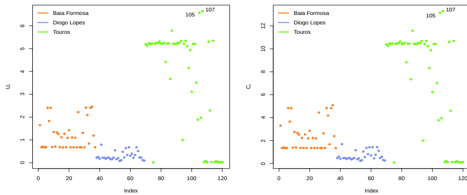
Figure 9: Index plots for \theta (response perturbation): (a) d_{max} and (b) total local influence.
