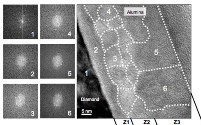
Figure 3. Low magnification HREM micrograph of sample B. On the left side the Fast Fourier transforms (FFTs) from six areas (labeled from 1 to 6) of the micrograph on the right are showed as an example of all those obtained on the whole micrograph. Three zones, labeled Z1, Z2, and Z3, are identified. Z1 corresponds to amorphous alumina (FFT 2), while Z2 and Z3 correspond to polycrystalline cubic alumina (FFT 3, 4, 5 and 6) where dashed white lines are used to delimit grains with different orientations.
