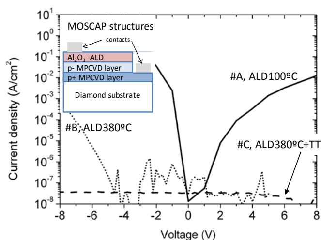
Figure 1. Representative I/V characteristics of the three samples under positive and negative bias. Sample A (ALD 100 °C) showed strong leakage current under positive and negative biases, while for sample B (ALD 380 °C), the leakage was strongly reduced, and sample C (ALD 380 °C + annealing at 500 °C for 30 min) showed no leakage current. MPCVD: microwave plasma-assisted chemical vapor deposition.
