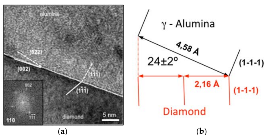
Figure 4. (a) HREM micrograph of sample C, where a fully crystalline alumina layer is observed. Lines and dashed lines were used to indicate where the (\bar{1}\bar{1}\bar{1}) planes are in both diamond and alumina crystals. The insets correspond to the FFTs of both materials; (b) Schematic representation of the (\bar{1}\bar{1}\bar{1}) planes' correspondence at the diamond/alumina interface in sample C.
