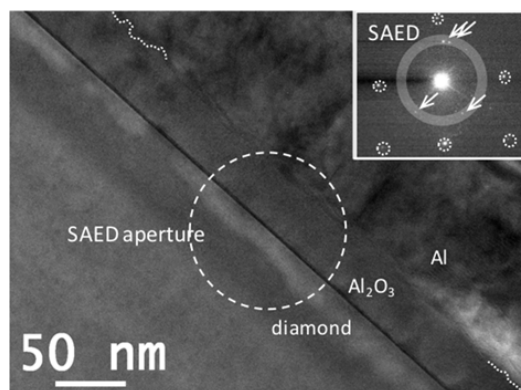
Figure 2. High-resolution electron microscopy (HREM) micrograph of sample A, where the followings is observed: The alumina layer is polycrystalline; Non-planar alumina top surface (dashed white line marks the top surface of the alumina in a specific area of the micrograph); and There is a thin layer of amorphous alumina between the diamond and the polycrystalline alumina area (identified by the white arrow).
