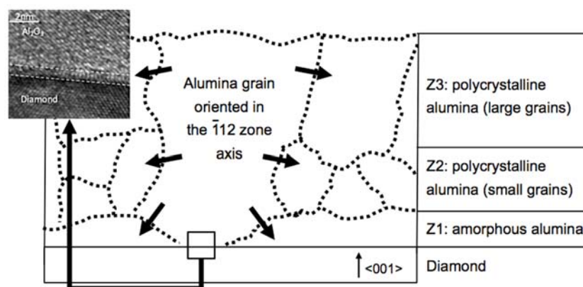
Figure 5. Schema of the grain evolution on \gamma -alumina grown on a diamond by ALD. The inset is a HREM micrograph of the alumina–diamond interface when amorphous alumina was not observed.
