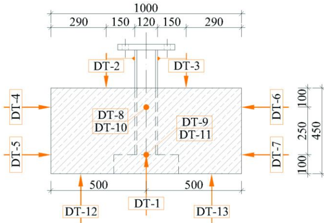
Fig. 6. Scheme of the implemented displacement transducers in CoPOT, south face view.
