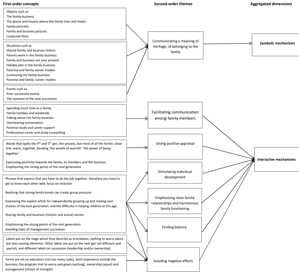
Figure 1: Data structure
